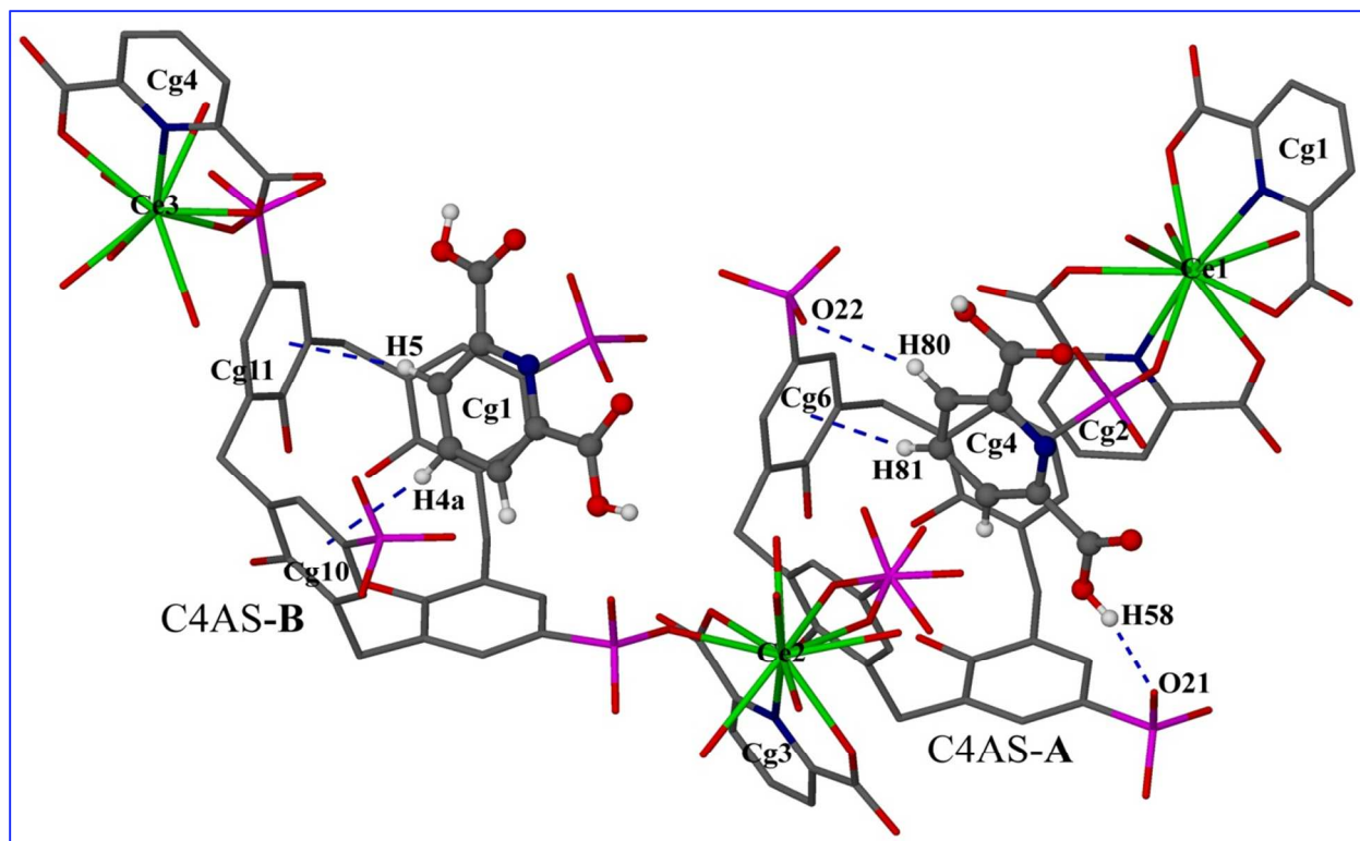
Figure 3. Displaying inclusion of pyridyl rings of the PDA ligands by C-H \cdots\pi , C-H \cdots O and O-H \cdots O interactions. Atoms of pyridyl rings inserted into the cavity are shown as spheres of arbitrary radii. Blue broken lines depict CH \cdots\pi , CH \cdots O(S) and OH \cdots O(S) interactions.
