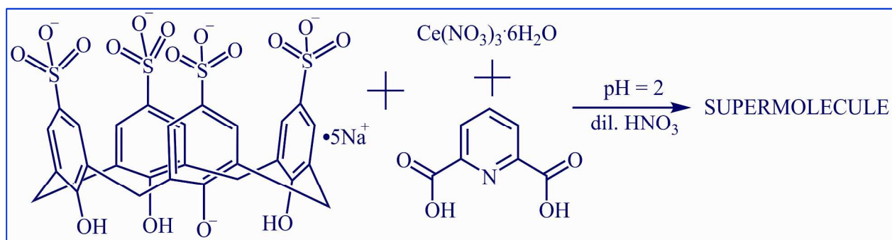
Scheme 1 Preparation of supermolecule.
