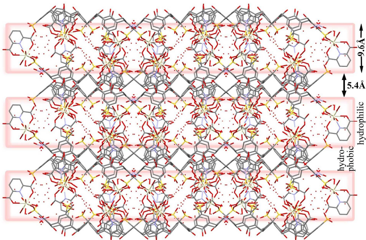
Figure 8 Display of hydrophilic and hydrophobic layers.
