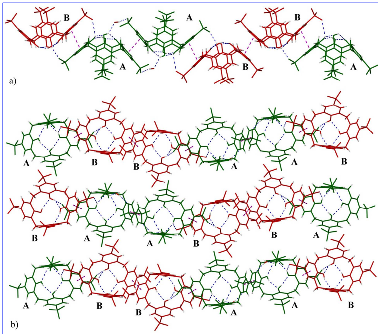
Figure 7 a) A view of the zig-zag chains running parallel to b -axis (C4ASs-A in green and C4ASs-B in red). b) The extended (along c -axis) structure of 1 showing ‘up-down’ antiparallel bilayer arrangements (AABBAABB.....). The hydrogen bonding between hydroxyl groups and sulfonate groups are shown as dashed blue lines while \pi - \pi interactions shown as dashed pink lines.
