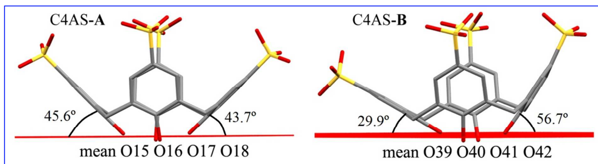
Figure 5 Display of two splayed p -sulfonatocalix[4]arenes in supermolecule 1.
