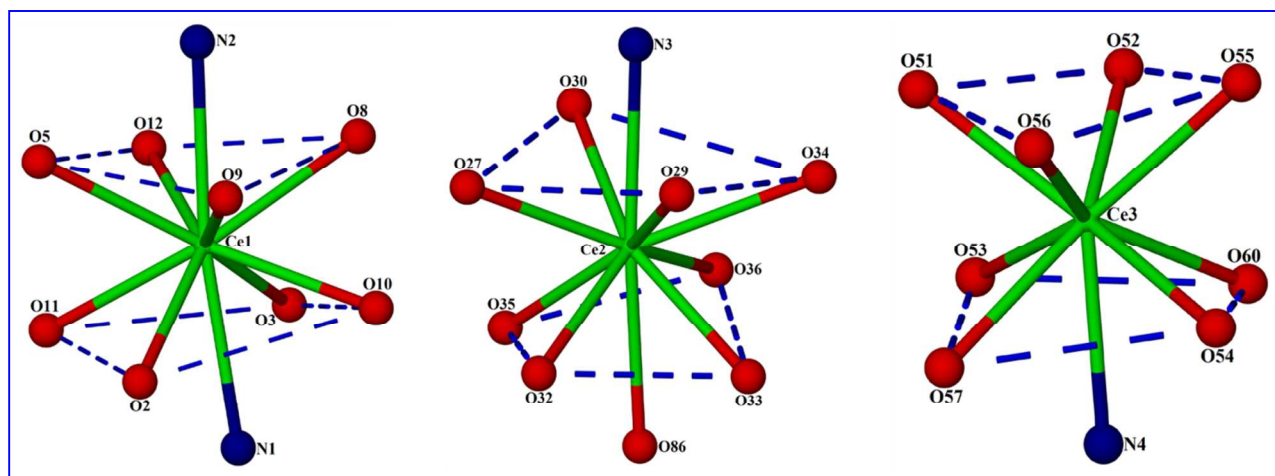
Figure 2. Display of distorted capped square antiprisms of all the three Ce(III) coordination environment.
