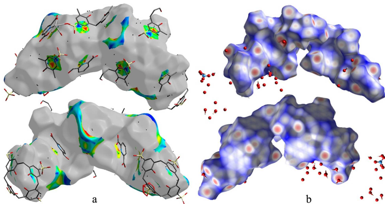
Figure 9 Front and back views of the Hirshfeld surfaces representation for 1 mapped with (a) shape-index and (b) d_{\text{norm}} with all types of intermolecular interactions considered.
