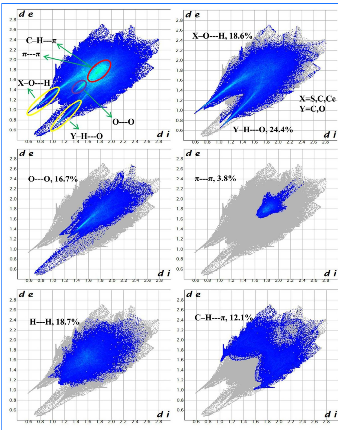
Figure 10 Fingerprint plots of 1 : all contacts accounted for (upper left) and resolved into different intermolecular interactions showing the percentages of contacts contributing to the total Hirshfeld surface area of molecules.
