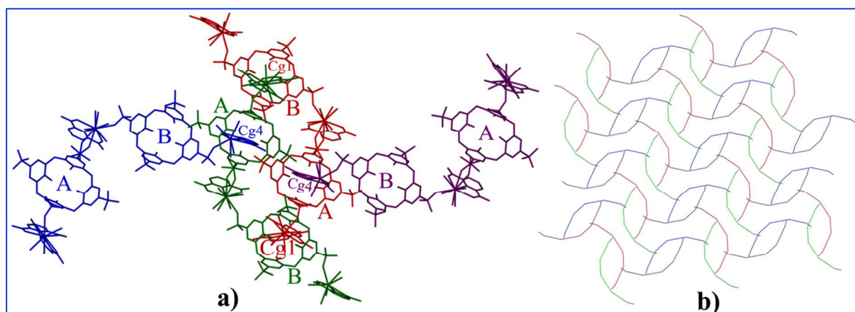
Figure 4 a) Projection of four supermolecules of 1 in the unit cell. The four symmetry-related molecules are represented in different colours and hydrogen atoms have been removed for clarity. b) Schematic representation of repeating pattern of the four supermolecules.
