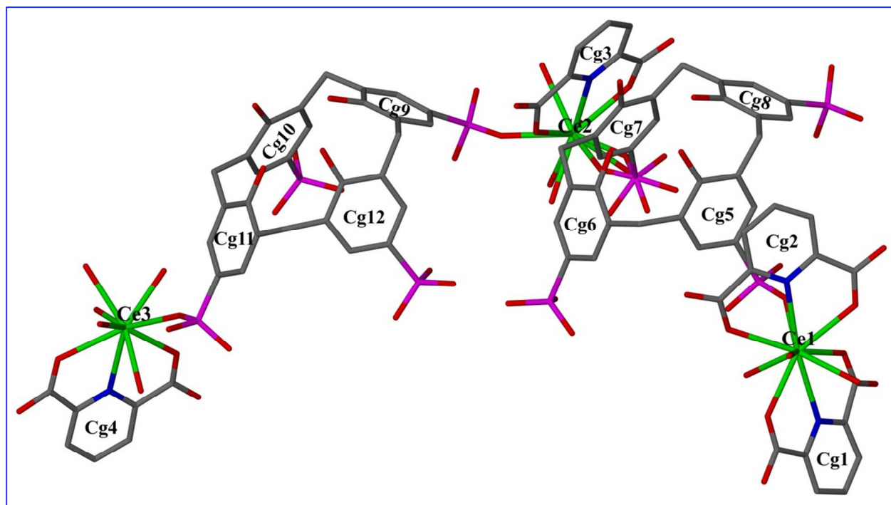
Figure. 1 Asymmetric unit displaying C-shaped supermolecule 1 . Water molecules, nitrate anion and H-atoms have been omitted for clarity. Aromatic rings have been numbered to show centre of gravity. Disorder of the sulfonate group on Cg7 is shown.
