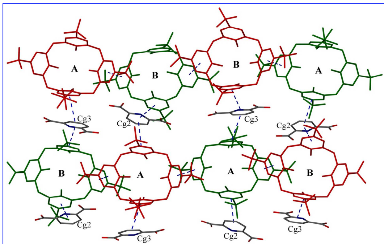
Figure 6 Alternately upwards and downwards arrangement of C4ASs displaying sandwiched pyridyl rings between the aryl rings of C4ASs. Broken lines depict \pi --- \pi interactions. Upward-pointing molecules (red) and the downward-pointing molecules (green).
