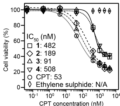
Fig. 4 Cytotoxicity study (48 h incubation) comparing free CPT, 1 , 2 , 3 , 4 and ethylene sulphide against the MCF-7 breast cancer cell line. Cell viability was determined by SRB assay and data are presented as mean ± s.d. ( n = 3).
