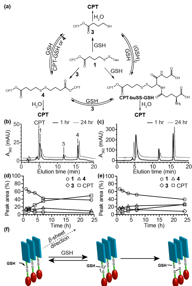
Fig. 2 GSH-induced release of CPT from 1 . CPT-containing reaction products formed and the exchange reactions that can occur during the GSH-induced reduction of 1 (a). HPLC analysis of GSH-induced release of CPT from DA 1 at 5 (b) and 50 \mu\text{M} (c) in 10 mM sodium phosphate containing 10 mM GSH at 37 ^{\circ}\text{C} after 1 and 24 h. Peak areas of the 4 main species (expressed as percentages of the total area; the area for 4 was halved to reflect the increased absorbance due to two CPT molecules) showing the evolution over time for the 5 (d) and 50 \mu\text{M} (e) solutions of 1 . Possible mechanism for the formation of the disulphide dimer 4 within nanofilaments or smaller \beta -sheet aggregates (f).
