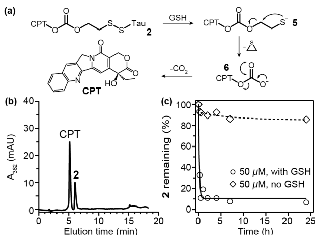
Fig. 3 (a) Mechanism of GSH induced release from 2 . (b) HPLC analysis of a solution with 2 (50 μM) and 10 mM GSH in 10 mM sodium phosphate after 50 min at room temperature. (c) Degradation of 2 (50 μM) with or without 10 mM GSH in 10 mM sodium phosphate at 37 °C.
