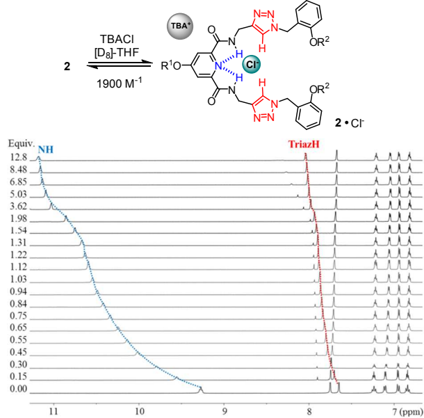
Fig. 1 Stacked partial 1 H NMR spectra ([D 8 ]-THF, 700 MHz) of compound 2 upon addition of TBACl.
