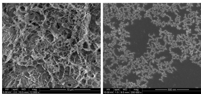
Fig. 5 SEM image of freeze-dried sample of 1 in 12 K magnification (left) and air-dried polymer 1 - \text{Cl}^- complex from toluene at 200 K magnification (right).
