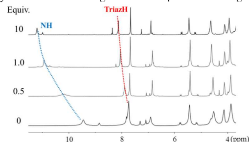
Fig. 3 Stacked partial 1 H NMR ([D 8 ]-THF, 400 MHz) spectra of 1 upon addition of TBACl.
