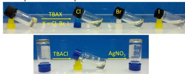
Fig. 4 (top) Gel-to-sol responsive behaviour of polymer toluene gel 1 upon addition of TAB salts of halide. (bottom) Sol-to-gel responsive behaviour of polymer 1 -Cl - complex upon addition of AgNO 3 salt.
