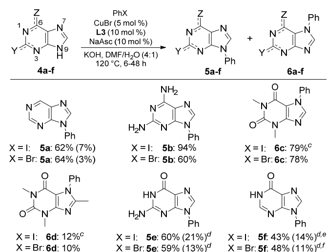
Scheme 2 Coupling of Iodobenzene/Bromobenzene to Various Purines a,b
