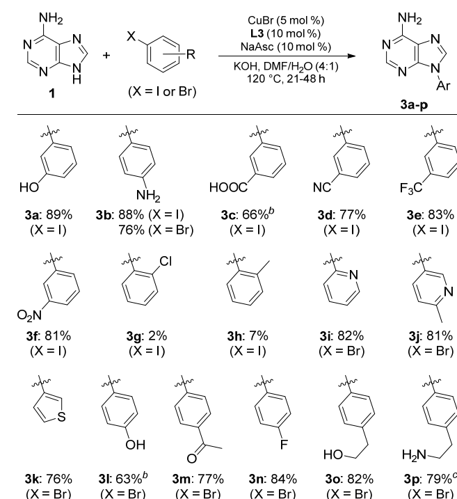
Scheme 1 Coupling of Various Aryl Halides to Adenine a
