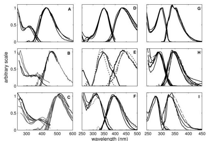
Figure 2: Excitation (left) and emission (right) spectra of widely distributed PARAFAC components in the OpenFluor database. A-F are humic-like components and G-I are protein-like. (A) C_{320/420} ; (B) C_{370/460} and C_{345/460} ; (C) C_{400/518} nm and C_{380/500} nm; (D) C_{350/430} in five water treatment plant models from a single study; (E) qualitatively similar components to C_{350/430} in other studies; (F) C_{320/400} ; (G) C_{300/340} displaying fine structure in the emission spectrum; (H) C_{295/356} correlated to lignin in one study; and (I) C_{275/350} , similar to free dissolved tryptophan.
