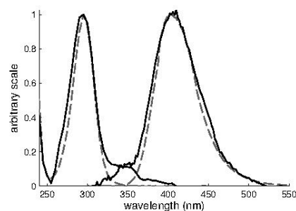
Figure 3: Fluorescence spectra of a terrestrially derived PARAFAC component in the nearly pristine Mackenzie River watershed 30 (lines) compared with pure dissolved sodium salicylate (dashes).
