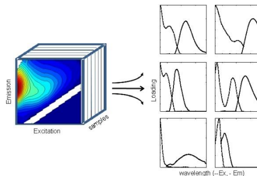
Figure 1: A dataset of fluorescence excitation emission matrices (EEMs) decomposed into six underlying components using PARAFAC.
