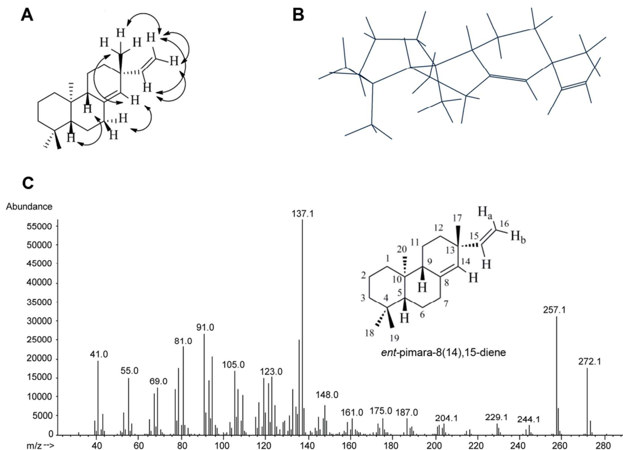
Figure 6. (A) Selected NOESY correlations and (B) a 3D representation of ent -pimara-8(14),15-diene. (C) Structure and mass spectrum of pure ent -pimara-8(14),15-diene.
