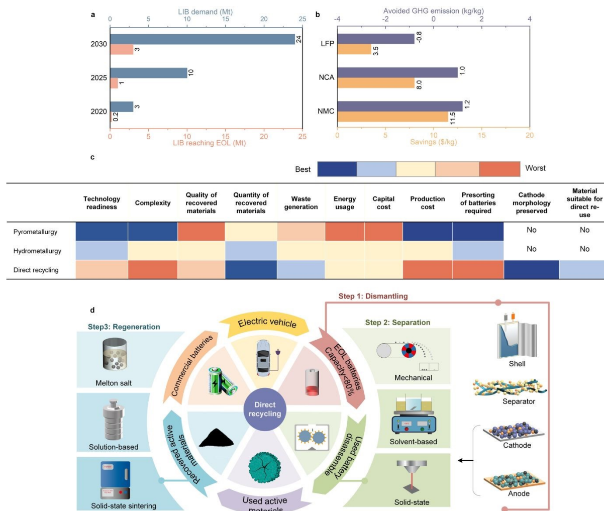
Fig. 1 (a) The projected LIB demand (Mt) and predicted LIB reaching EOL from 2020 to 2030 1-3 . (b) Savings ($/kg) and avoided GHG emissions (kg/kg) by recycling NMC, nickel cobalt aluminum oxide (NCA), and LFP 1, 4, 5 . (c) the comparison among pyrometallurgy, hydrometallurgy, and direct recycling. Adapted from Ref 5 . Copyright 2019 Springer Nature. (d) Illustration of the direct recycling workflow.
