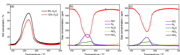
Fig. 6 Pd/MnTiO 2 and Cu/SSZ-13 monolith catalysts in series; (a) NO conversion profiles of 1 wt% Pd/MnTiO 2 + 2 wt% Cu/SSZ-13 with 5% water and 12% water contents and the effluent gas concentration profiles with (b) 5% water and (c) 12% water (GHSV = 20 000 h -1 (STP); gas inlet: 500 ppm NO, 5000 ppm H 2 , 10% O 2 , and 5/12% H 2 O balanced in Ar; T: 80–500 °C heating rate: 5 °C min -1 ).
