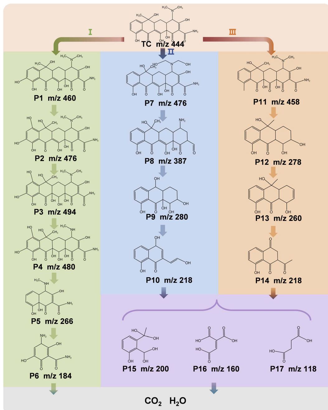
Fig. 6 The potential degradation pathways of TC in the NiFe–N–C/PMS process.
