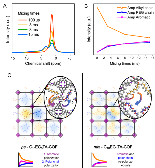
Fig. 6 (A) Projections from 2D ^1H - ^1H spin-diffusion ssNMR spectra at different mixing times. (B) Deconvolution results from Lorentzian curves. (C) Schematic representation of the proposed magnetization pathways: pathway A: starting from the alkyl chain, the magnetization crosses the aromatic framework before reaching the EG chain. Pathway B: starting from the alkyl chain the magnetization crosses directly to the EG chain; small insets describe the idealized behavior for pathway A (left) and pathway B (right). In a phase separated situation the pathway A should dominate and the transfer to EG would be delayed, leading to a slower increase of the blue signal compared to the pink one.
