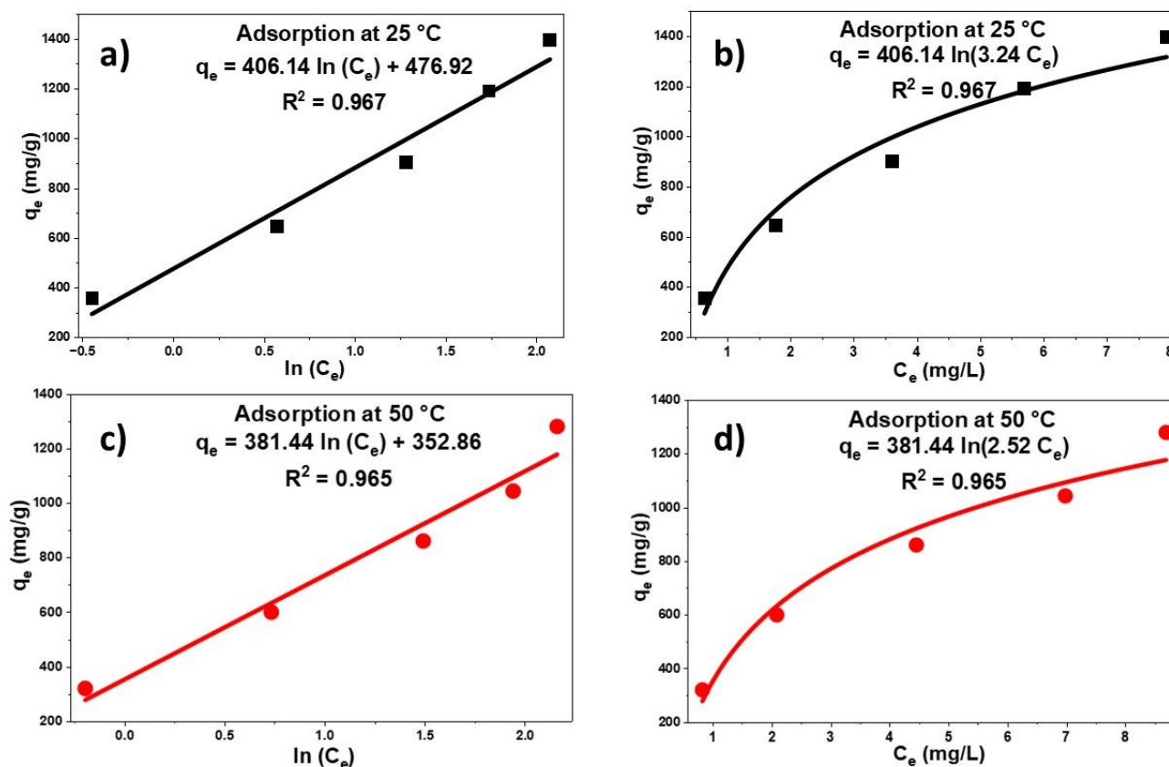
Fig 3 (a) Linear fit of the Temkin isotherm at 25 °C; (b) Non-linear fit of the Temkin isotherm at 25 °C; (c) Linear fit of the Temkin isotherm at 50 °C; (d) Non-linear fit of the Temkin isotherm at 50 °C.
