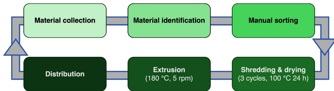
Figure 2. Holistic view of the PLA recycling process of the FilUM initiative.
