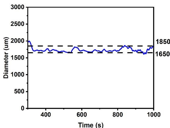
Figure 3. Filament diameter as a function of time for the blue recycled PLA extruded at 180 °C with a screw speed of 5 rpm. The dotted black lines represent the upper and lower acceptable limits of print quality filament diameter.
