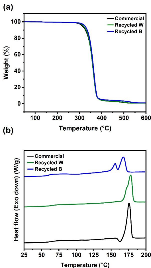
Figure 5. a) Thermogravimetric analysis of the prepared recycled filaments showing the weight % as a function of temperature. b) First heating curve of a DSC experiment of the prepared recycled filaments showing the heat flow as a function of temperature. W and B stands for the white and the blue recycled filament, respectively.
