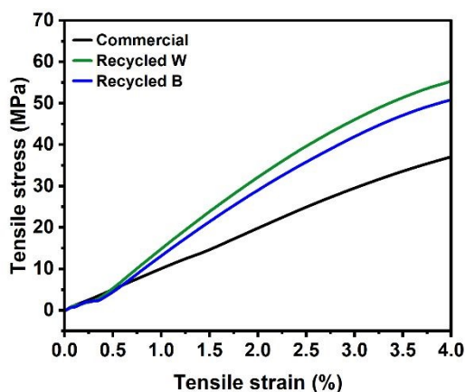
Figure 6. Representative tensile stress as a function of tensile strain for the commercial and recycled filaments. This region was used to determine the Young's modulus of the materials. W and B stands for the white and the blue recycled filament, respectively.
