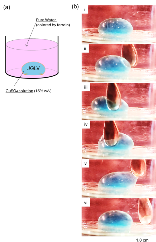
Fig. 2 Stability of UGLV against mechanical stimulus. (a) Schematic of a UGLV containing a 15% w/v \text{CuSO}_4 solution (blue color) surrounded by a ferriox-colored aqueous solution. The vesicle is situated in a pure water solution, \rho = 1.00 \text{ g cm}^{-3} . (b) Snapshots of the UGLV mechanically perturbed by a spatula. The UGLV retains the closed stable state against mechanical agitation. The interval for the images between (i) and (vi) is ca. 2 s. See the original movie in the SI, Video S2.
