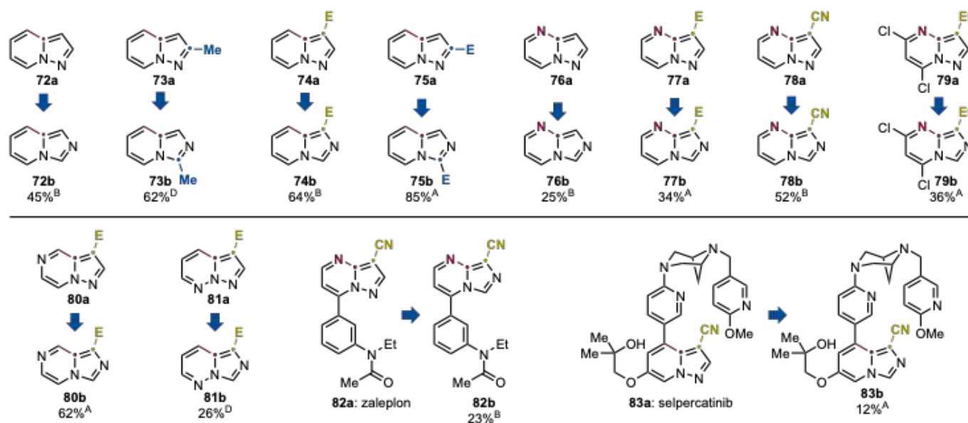
Scheme 6. Substrate scope for the pyrazole to imidazole conversion using pyrazolo[1,5-a]azine derivatives. A–D see Scheme 3 for the legend with the specific conditions used.
