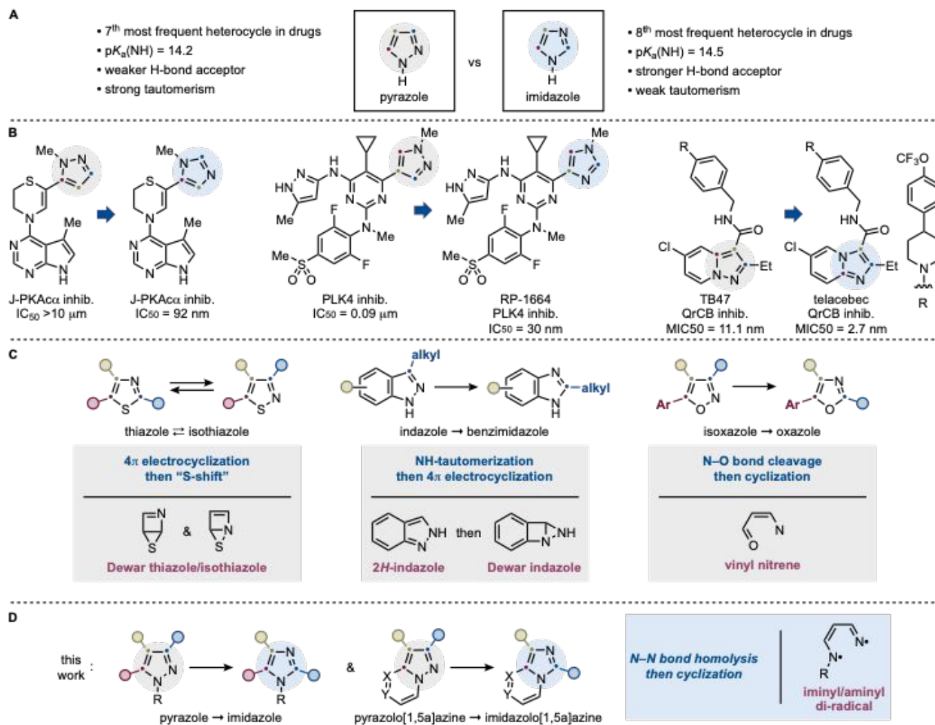
Scheme 1. A. Pyrazole and imidazole are two relevant N-heteroaromatics, but their N-atom dispositions provide key chemical difference. B. Examples of pyrazole \rightarrow imidazole conversions leading to improved bioactive molecules. C. Previous permutation work on other azoles features mechanistically distinct pathways and intermediates. D. This work demonstrates a direct pyrazole \rightarrow imidazole conversion that can be applied to pyrazolo[1,5a]azines.
