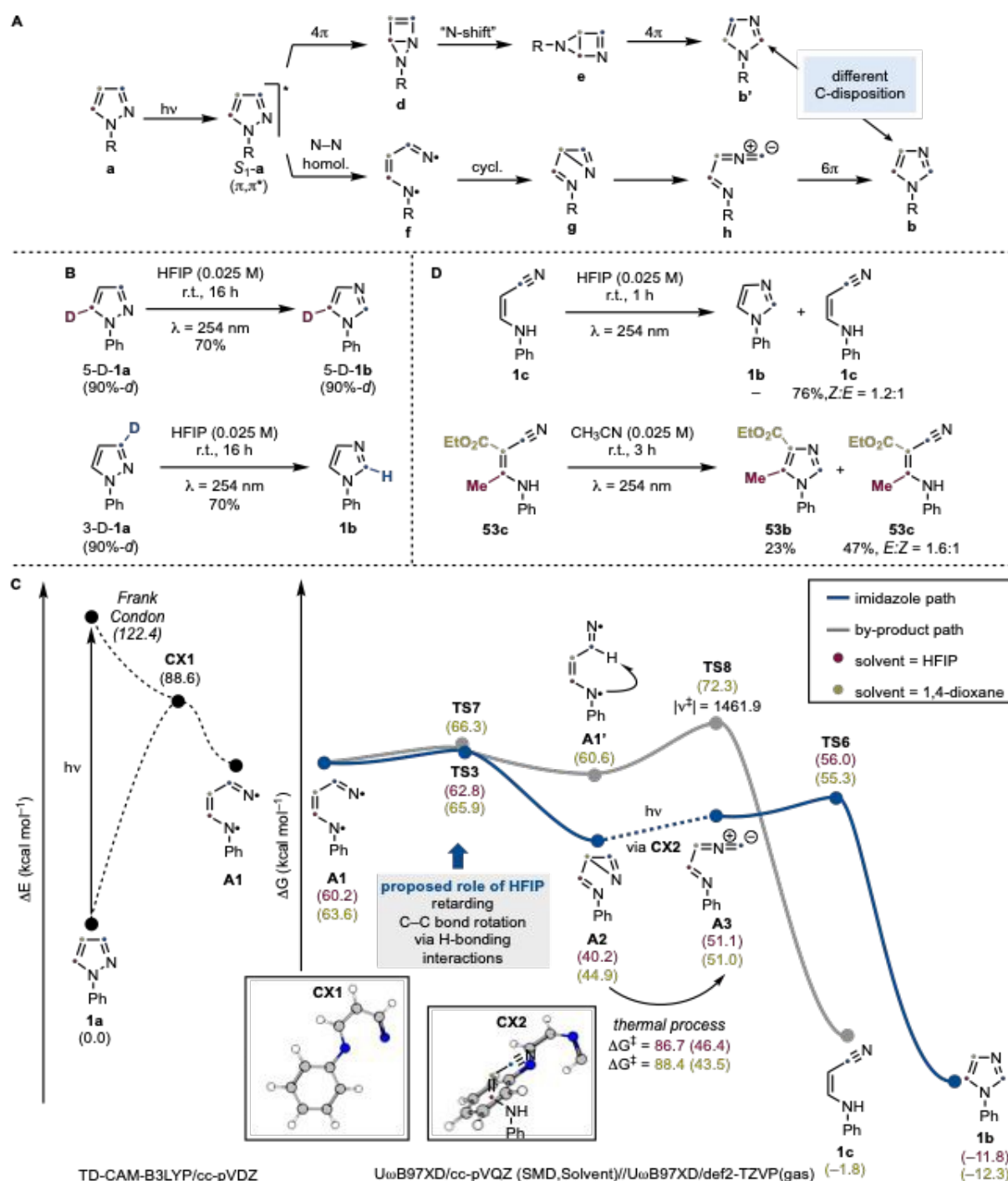
Scheme 8. A. Proposed mechanistic pathway for the pyrazole-imidazole conversion and computational studies. B. Experiments on deuterated 1a . C. Computational profile for the conversion of 1a into 1b and 1c . All energy values are in kcal mol -1 . D. Photochemical experiments on the reactivity of enamine nitriles by-products.
