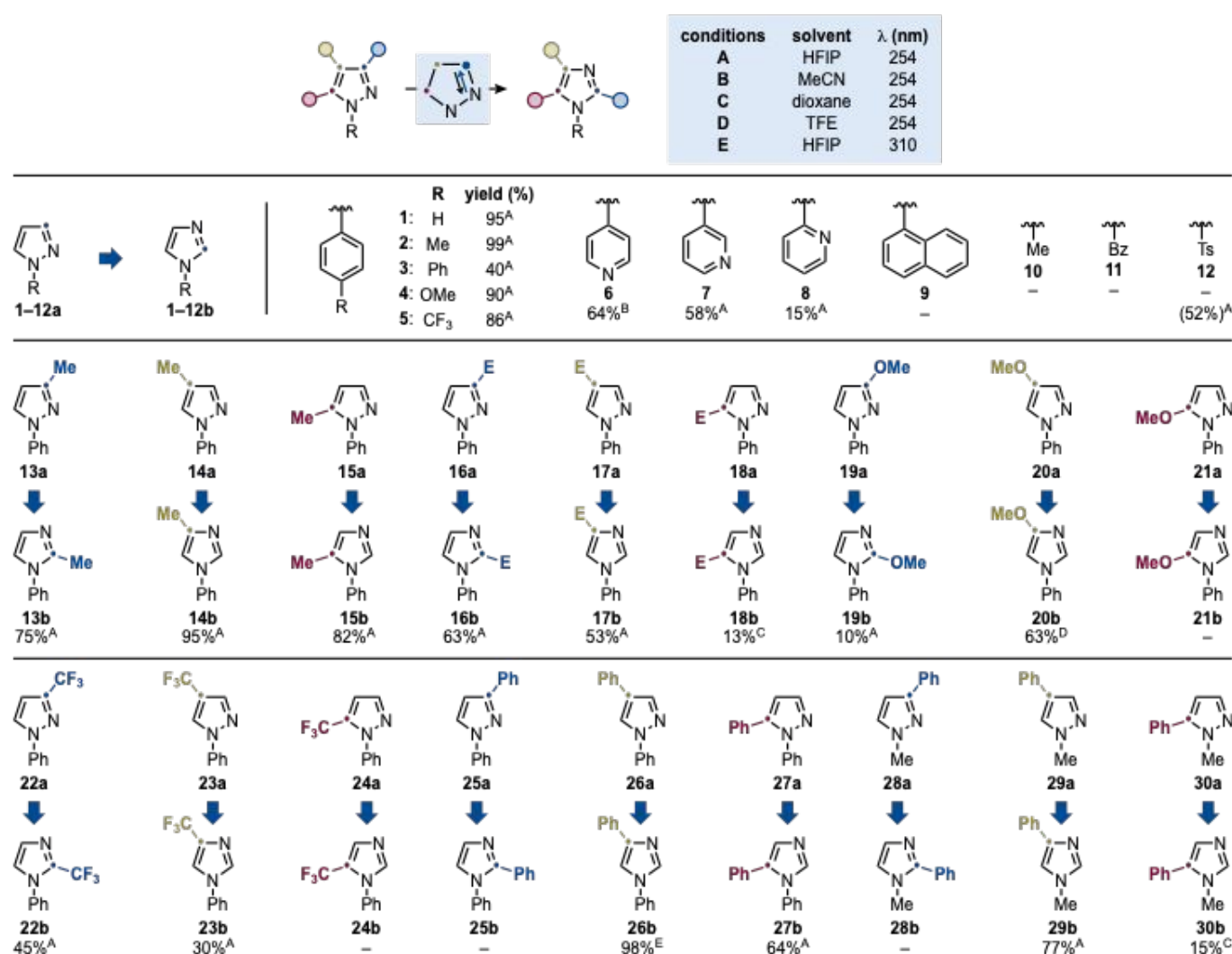
Scheme 3. Substrate scope for the pyrazole-to-imidazole conversion using mono-substituted derivatives. E = CO 2 Me. The yield for substrate 12 corresponds to the detosylated product.
