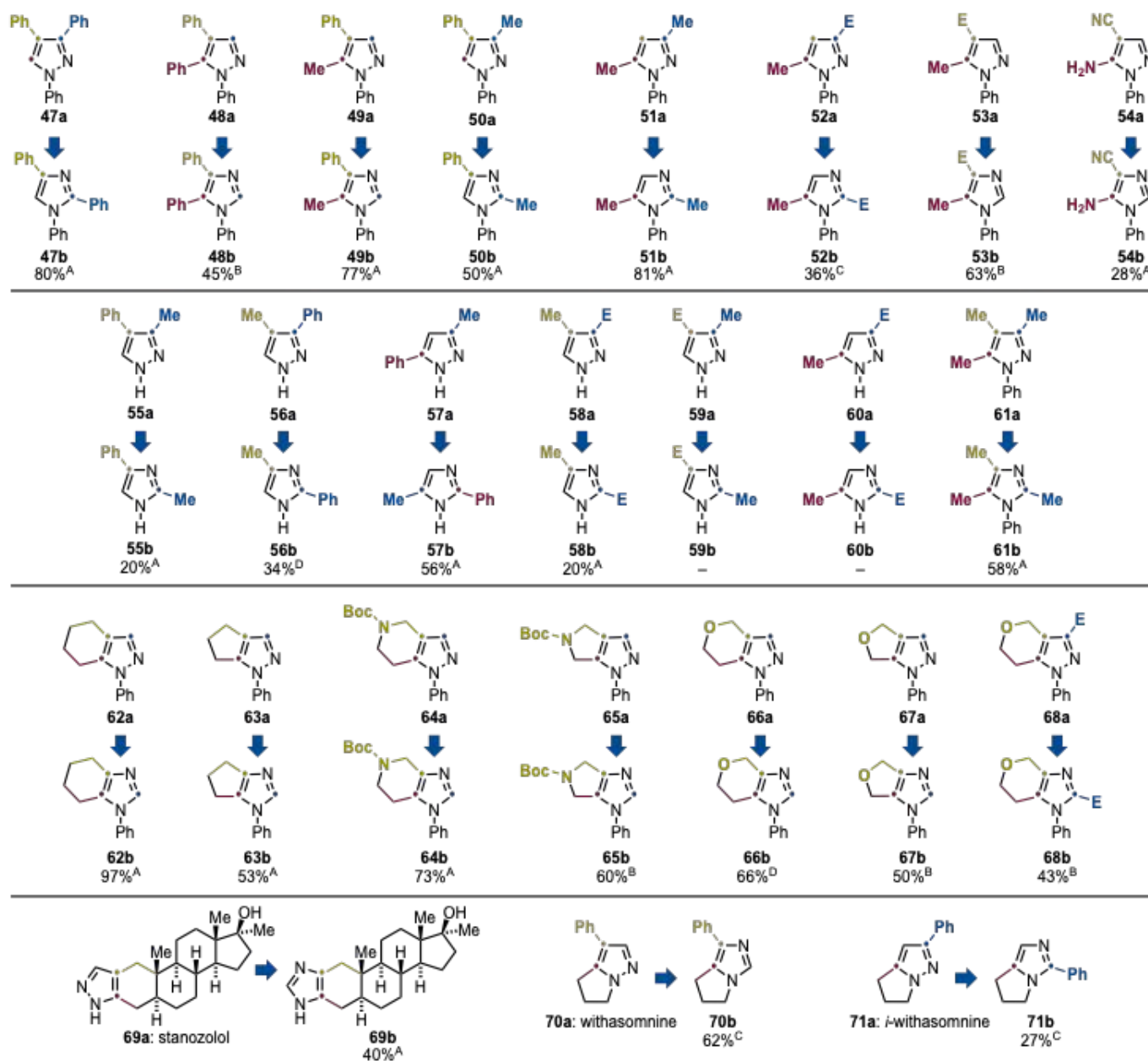
Scheme 5. Substrate scope for the pyrazole-imidazole conversion using di- and tri-substituted derivatives. A–D see Scheme 3 for the legend with the specific conditions used.
