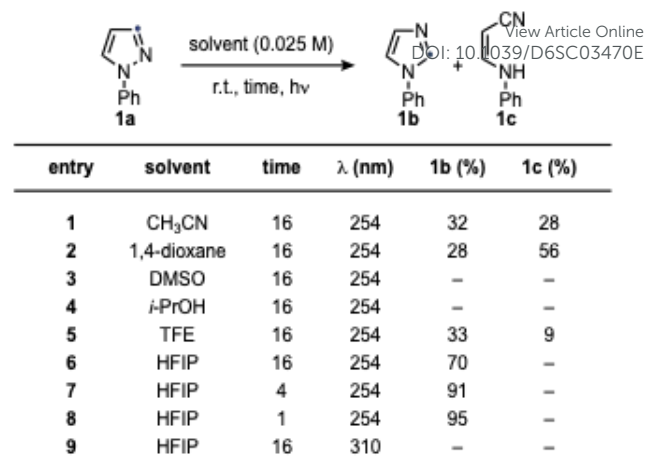
Scheme 2. Optimization of the pyrazole-to-imidazole conversion using 1a .
