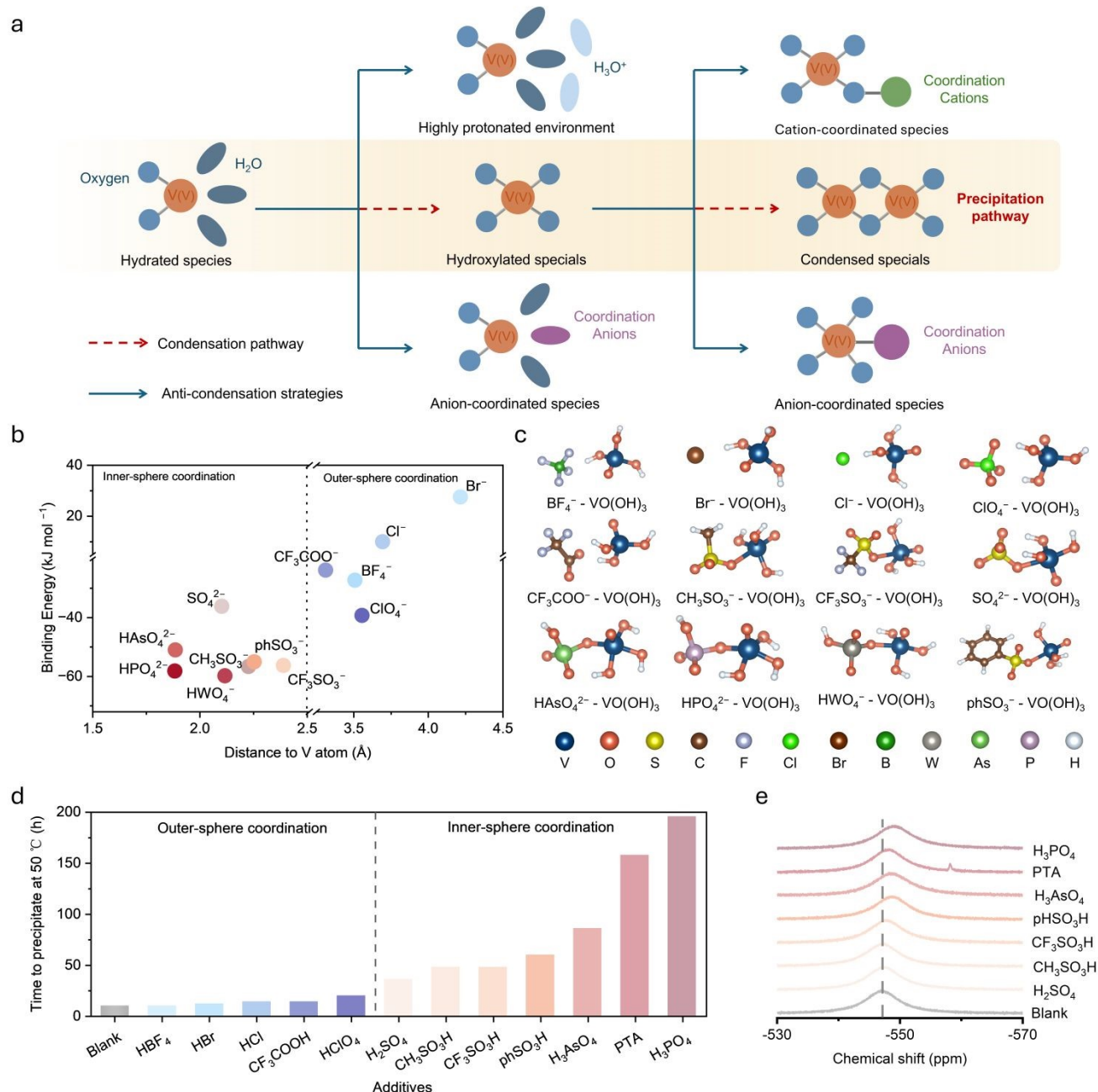
Figure 5. Anion coordination inhibition strategy. (a) Transformation pathway from solvated to precipitated species and strategies to overcome precipitation via high protonation environment and anion coordination. (b) Binding energy versus V-anion distance for 12 anions with VO(OH) 3 , with dashed line separating inner-sphere (<2.5 \text{\AA} ) and outer-sphere (>2.5 \text{\AA} ) coordination regions. (c) Optimized structures of anion-VO(OH) 3 complexes showing different coordination modes. (d) Experimentally measured precipitation time at 50 °C with different acid additives. (e) ^{51}\text{V} NMR chemical shift spectra showing significant shifts with inner-sphere coordinating anions.
