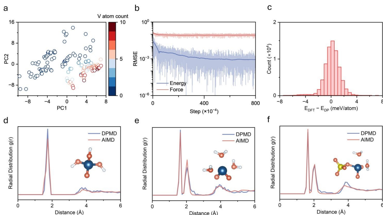
Figure 2. Deep potential model validation. (a) Principal component analysis showing structural diversity of training dataset with colors indicating vanadium atom count. (b) Root mean square error evolution for energy and force during training. (c) Error distribution histogram between DFT and DP predicted energies. (d-f) Radial distribution function comparison between DPMD and AIMD for (d) VO(OH) 3 , (e) [VO 2 (H 2 O) 3 ] + , and (f) [VO 2 (H 2 O) 2 SO 4 ] - , with insets showing representative local coordination structures.
