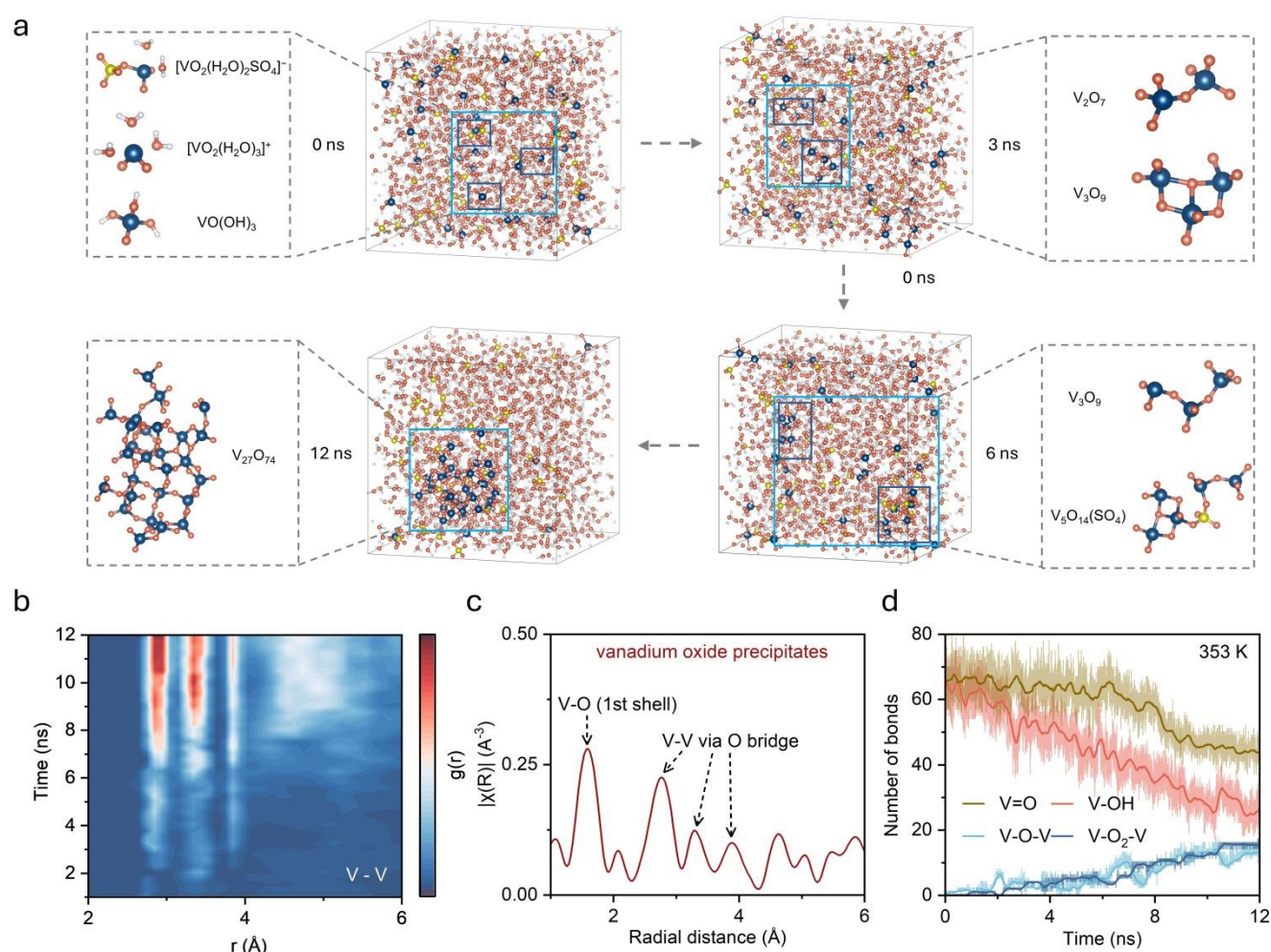
Figure 3. Kinetic evolution of pentavalent vanadium precipitation. (a) Representative snapshots from 12 ns DPMD simulation showing the transformation of \text{V}(\text{V}) species from monomers to polynuclear clusters, with magnified views of local structural evolution. (b) Time-resolved V-V RDF heatmap showing increasing intensity in the 2-6 Å range, indicating formation of oxygen-bridged vanadium species. (c) Fourier-transformed EXAFS spectrum |\chi(R)| of \text{V}(\text{V}) precipitate. (d) Evolution of different coordination bond types over time, with \text{V}=\text{O} and \text{V}-\text{OH} decrease while \text{V}-\text{O}-\text{V} and \text{V}-\text{O}_2-\text{V} increase.
