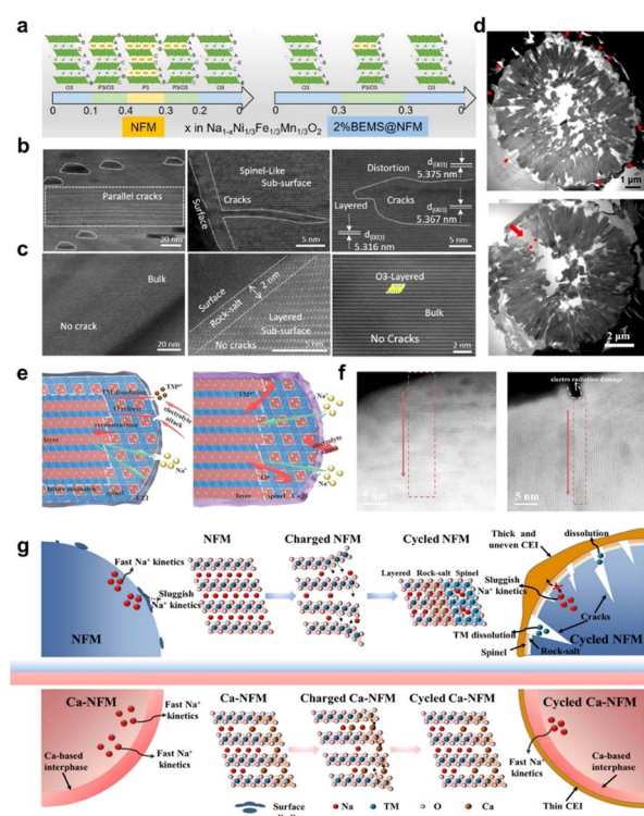
Fig. 14 (a) Phase structure evolution of 2% BEMS@NaNi 1/3 Fe 1/3 Mn 1/3 O 2 during charging and discharging cycles; HAADF-STEM images for (b) O3-NaNi 1/3 Fe 1/3 Mn 1/3 O 2 and (c) 2% BEMS@NaNi 1/3 Fe 1/3 Mn 1/3 O 2 . Reprinted with permission from ref. 153 Copyright 2025, Elsevier. (d) TEM cross-sectional images of O3-NaNi 0.65 Co 0.08 Mn 0.27 O 2 @AlF 3 and O3-NaNi 0.65 Co 0.08 Mn 0.27 O 2 after 200 cycles. Reprinted with permission from ref. 154 Copyright 2018, American Chemical Society. (e) Schematic structural models and (f) HAADF-STEM images of O3-NaNi 1/3 Fe 1/3 Mn 1/3 O 2 and 1 wt%-Co x B@NaNi 1/3 Fe 1/3 Mn 1/3 O 2 . Reprinted with permission from ref. 155 Copyright 2024, John Wiley and Sons. (g) Schematic diagram of the structural evolution of NaNi 1/3 Fe 1/3 Mn 1/3 O 2 and Ca-NaNi 1/3 Fe 1/3 Mn 1/3 O 2 . Reprinted with permission from ref. 156 Copyright 2025, American Chemical Society.
