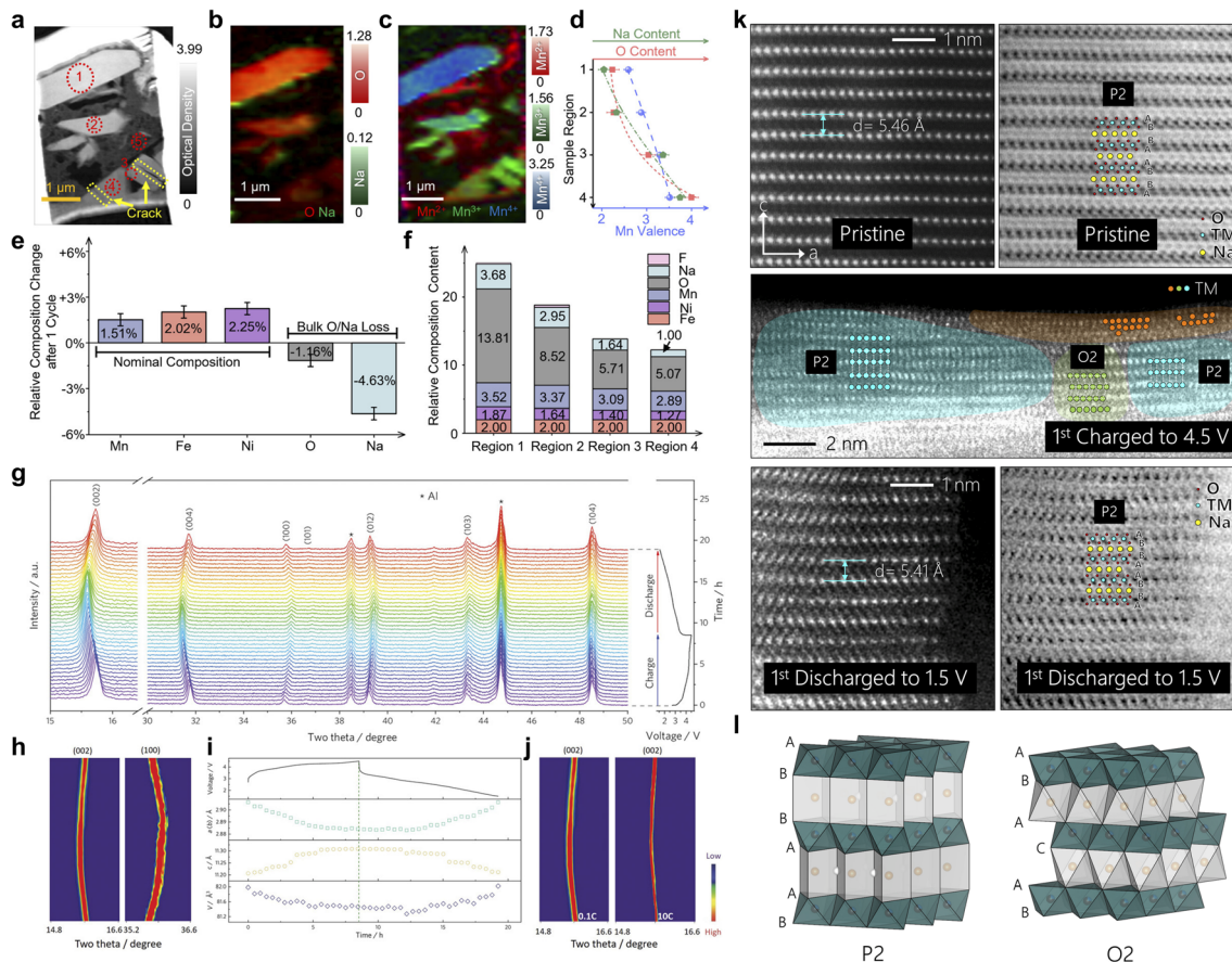
Fig. 4 (a) Averaged ptychography amplitude image from all elemental edges; color composite map of conventional STXM images from the (b) O and Na K-edge, (c) Mn^{2+} , Mn^{3+} , and Mn^{4+} edges; (d) trends in Mn oxidation states and distribution of O and Na content across different sample regions; (e) compositional changes in Mn, Fe, Ni, O, and Na after cycling; (f) quantitative XAS analysis in different regions. Reprinted with permission from ref. 54 Copyright 2025, American Chemical Society. (g) In situ XRD patterns of P2- Na_{0.7}Mg_{0.2}[Fe_{0.2}Mn_{0.6}\square_{0.2}]O_2 in the voltage range of 1.5–4.5 V (0.1C), along with (h) the corresponding contour plots and (i) evolution of lattice parameters; (j) contour plots of the evolution of the (002) peak at 0.1 and 10C. Reprinted with permission from ref. 55 Copyright 2021, John Wiley and Sons. (k) HAADF STEM images of Na_{0.72}[Li_{0.24}Mn_{0.76}]O_2 of different charge/discharge states on the particle surface; (l) schematic diagram of P2 and O2 structures. Reprinted with permission from ref. 56 Copyright 2019, Elsevier.
