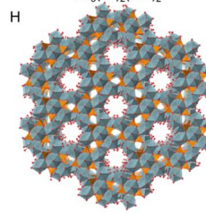
(H 2 O)[(UO 2 ) 4 (2-pmb) 2 (H 2 O) 3 ]·0.5H 2 O 2-pmbH 3 = 2-(phosphonomethyl)benzoic acid
