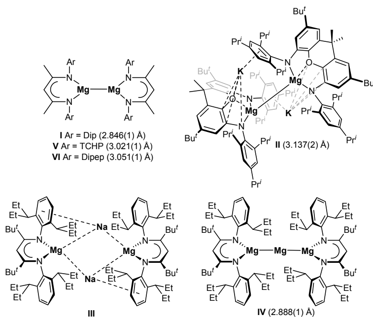
Figure 1. Previously reported examples of magnesium(I) and magnesium(0) compounds (Mg–Mg bond lengths in parentheses). Dip = 2,6-diisopropylphenyl, TCHP = 2,4,6-tricyclohexylphenyl, Dipep = 2,6-di(3-pentyl)phenyl.
