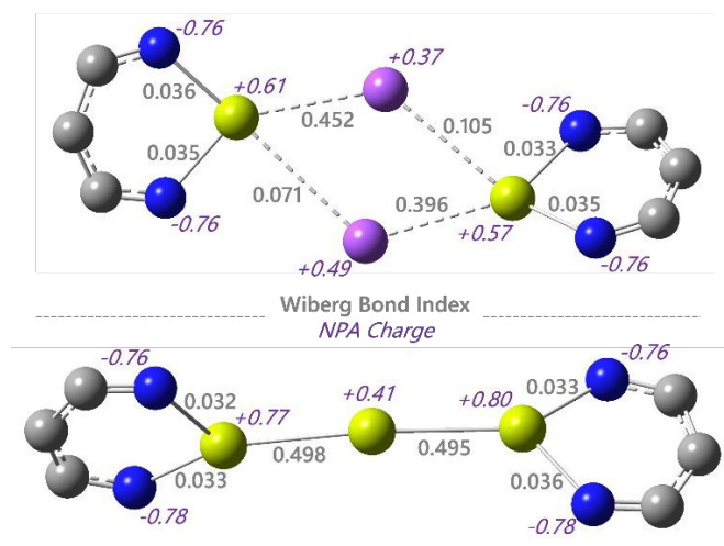
Figure 5. Select NBO data for 6 (top) and 8 (bottom). Wiberg Bond Indices (WBIs) are listed in bold, with natural population analysis (NPA) charge data in purple text. Colour code: carbon = grey; nitrogen = blue; magnesium = yellow; and sodium = purple. Tricyclohexylphenyl and tert -butyl groups omitted for clarity.
