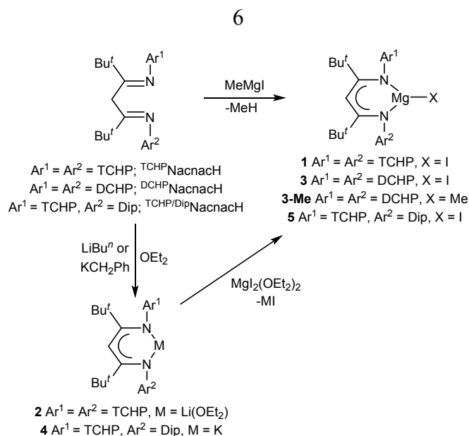
Scheme 1. Synthesis of compounds 1-5 ; DCHP = 2,6-dicyclohexylphenyl.
