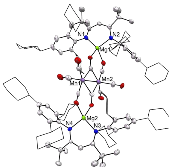
Figure 7. Molecular structure of 11 (25% thermal ellipsoids; hydrogen atoms omitted; cyclohexyl groups shown as wireframe for clarity). See text for relevant bond lengths.
