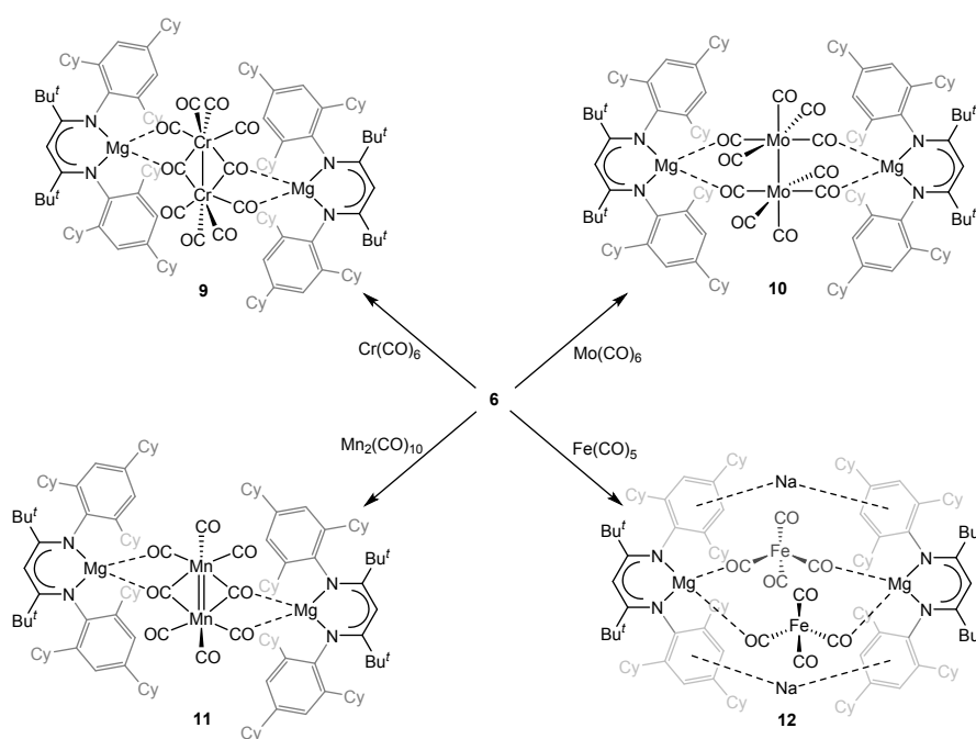
Scheme 3. Synthesis of compounds 9-12 .
