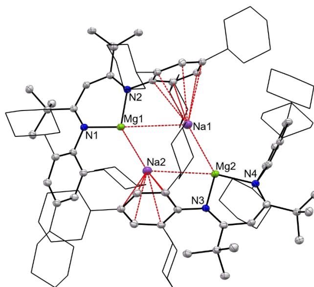
Figure 3. Molecular structure of 6 (25% thermal ellipsoids; hydrogen atoms omitted; cyclohexyl groups shown as wireframe for clarity). See text for relevant bond lengths.
