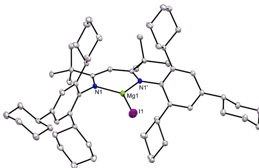
Figure 2. Molecular structure of 1 (25% thermal ellipsoids; hydrogen atoms omitted). Selected bond lengths (Å) and angles (°): I(1)-Mg(1) 2.5927(11), Mg(1)-N(1) 1.9984(18), N(1)-Mg(1)-N(1)' 97.40(10), N(1)-Mg(1)-I(1) 131.30(5).
