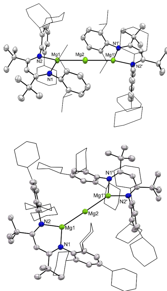
Figure 4. Molecular structures of 7 (top) and 8 (bottom) (25% thermal ellipsoids; hydrogen atoms omitted; cyclohexyl and isopropyl groups shown as wireframe for clarity). See text for relevant bond lengths and angles.
