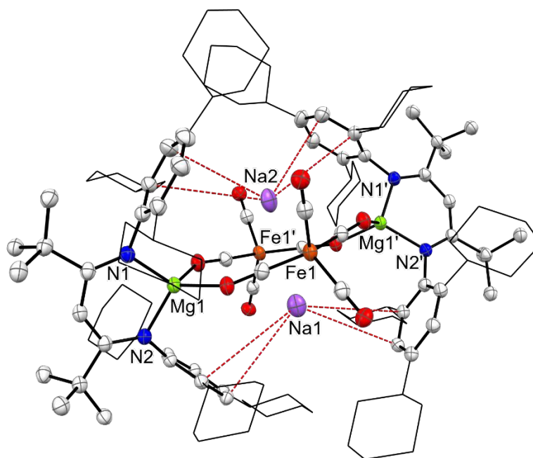
Figure 8. Molecular structure of 12 (25% thermal ellipsoids; hydrogen atoms omitted; cyclohexyl groups shown as wireframe for clarity).
