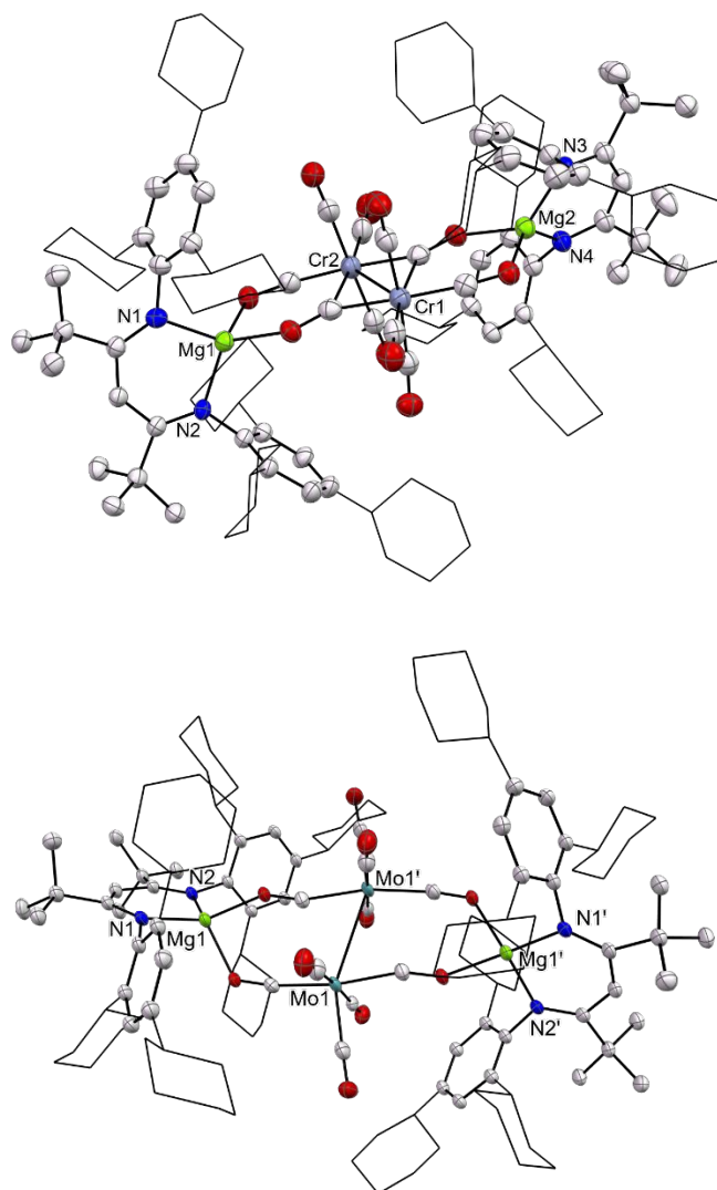
Figure 6. Molecular structures of 9 (top) and 10 (bottom) (25% thermal ellipsoids; hydrogen atoms omitted; cyclohexyl groups shown as wireframe for clarity). See text for relevant bond lengths.
