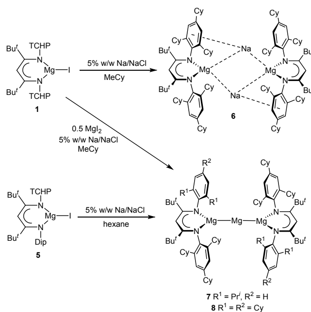
Scheme 2. Synthesis of compounds 6-8 .
