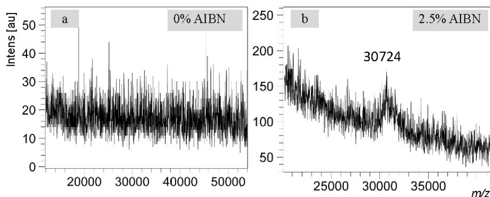
Figure 4. Application of eMALDI MS in real world research. RP HPLC purified 100-mer (6), which was synthesized on carbon fiber, was used for the analyses. MALDI samples were prepared using the improved protocol involving defined quantity of 3-HPA. ON quantity was 30 ng. Each spectrum was selected from the most representative ones from at least ten measurements. The data indicate that without AIBN, the 100-mer was not detectable (a). With 2.5% AIBN, unambiguous conclusion can be drawn that synthesis of ON on carbon fiber is feasible (b).
