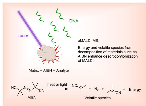
Figure 1. The concept of enhanced MALDI MS (eMALDI MS).
