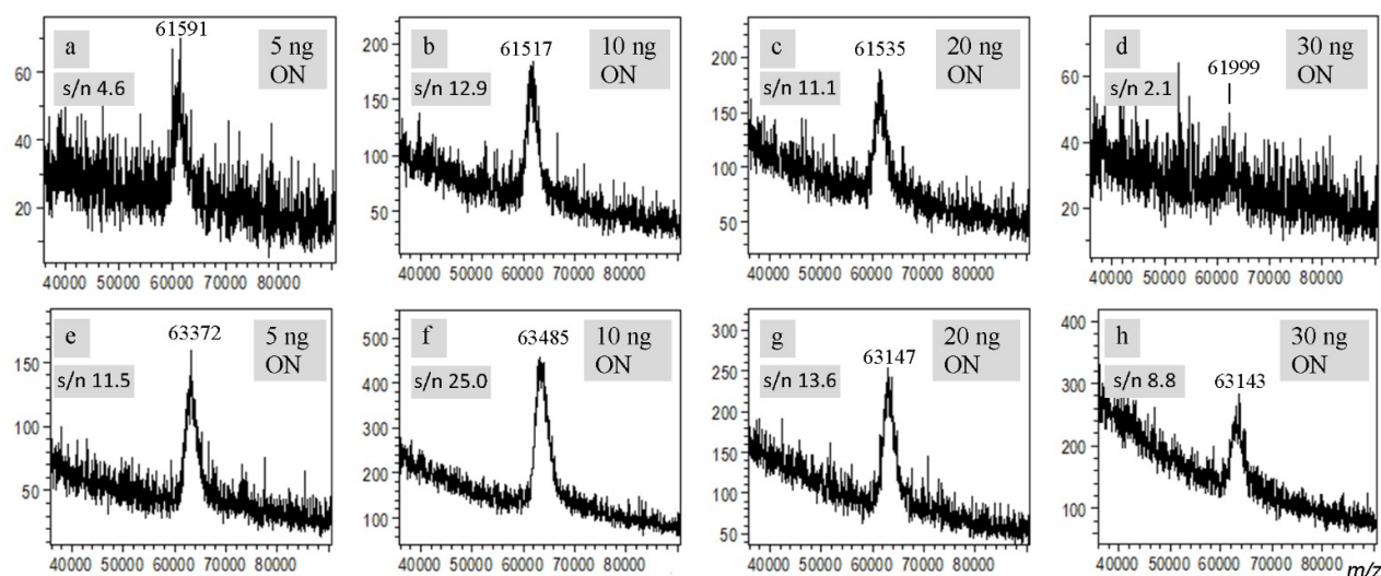
Figure 3. Effects of the quantity of ON on eMALDI MS. CBP and RP HPLC purified 200-mer ( 3 , a-d) and agarose gel electrophoresis and SPRI magnetic bead cleaned 202-mer ( 4 , e-h) were used for the analyses. MALDI samples were prepared using the improved protocol involving defined quantity of 3-HPA. AIBN concentrations were 2.5% for a-d and 3% for e-h. Each spectrum was selected from the most representative ones from at least five measurements. For the ds 202-mer ON 4 , only one peak is observable, instead of two, due to peak broadening caused by salt adducts and the relatively small mass difference between the two strands. The data indicate that suitable quantity of ON should be used for eMALDI MS.
