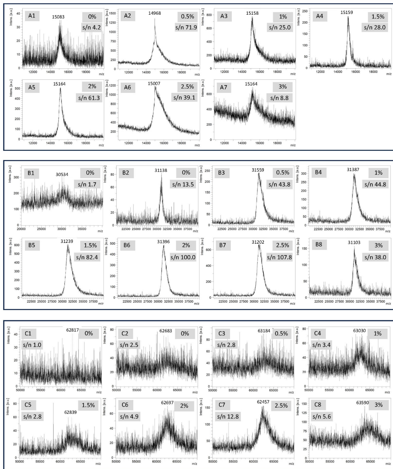
Figure 2. Effects of concentration of AIBN on the performance of MALDI MS analysis of ONs. A1-7: 50-mer ON (1) purified with CBP. B1-8: 100-mer ON (2) purified with CBP (for all) followed by RP HPLC (for B2-8). C1-8: 200-mer ON (3) purified with CBP (for all) followed by RP HPLC (for C2-8). ON quantity was ~5 ng. MALDI samples were prepared using the original protocol involving saturated 3-HPA. See experimental section for details. The percentage data such as 0% and 2% at the upper right corner of each spectra indicate the concentration of AIBN. Each spectrum was selected from the most representative ones from at least ten measurements. For each ON, the quality of the spectra exhibited a characteristic trend, poor at no or low AIBN, reaching an optimum at approximately 2% AIBN, and deteriorating once the AIBN concentration exceeded 2%. The trend is illustrated by the signal-to-noise (s/n) ratios versus AIBN concentrations in Figure S1. The theoretical molecular masses of ONs 1-3 are provided in the Supporting Information. The determined masses have significant deviations. Internal reference should be used when mass accuracy is crucial.
