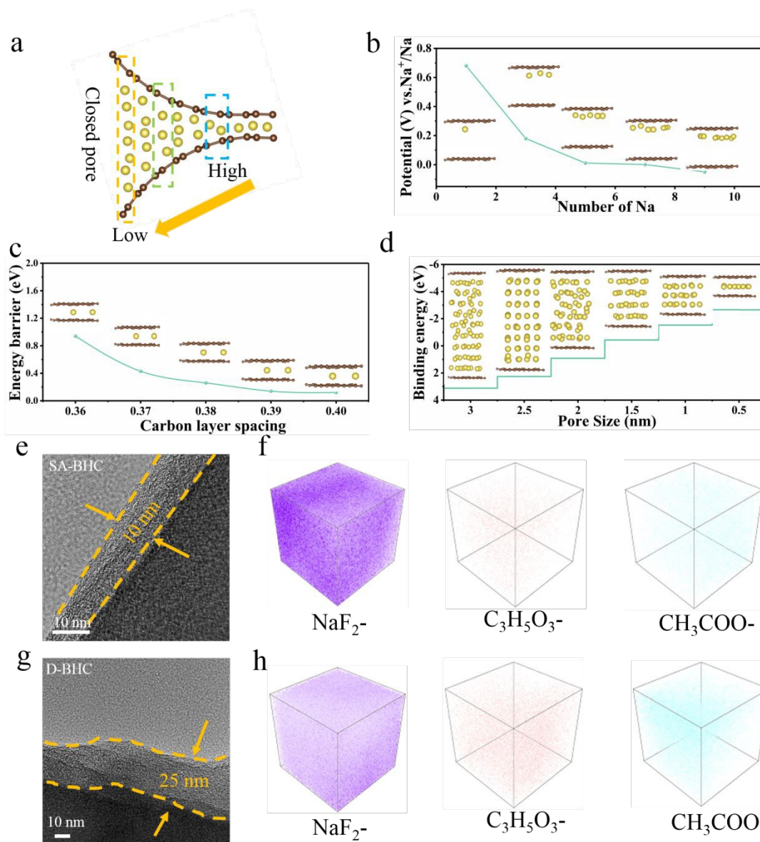
Fig. 5. (a) Schematic closed-pore model used for theoretical calculations. (b) Evolution of average potential during stepwise Na filling and corresponding optimized configurations. (c) Calculated \text{Na}^+ diffusion barriers as a function of carbon interlayer spacing. (d) Energetics of Na filling as a function of pore size. (e,g) HRTEM images of the SEI on SA-BHC (e) and D-BHC (g) electrodes after cycling. (f,h) 3D TOF-SIMS reconstructions showing the spatial distributions of representative inorganic and organic species in the SEI on SA-BHC (f) and D-BHC (h).
