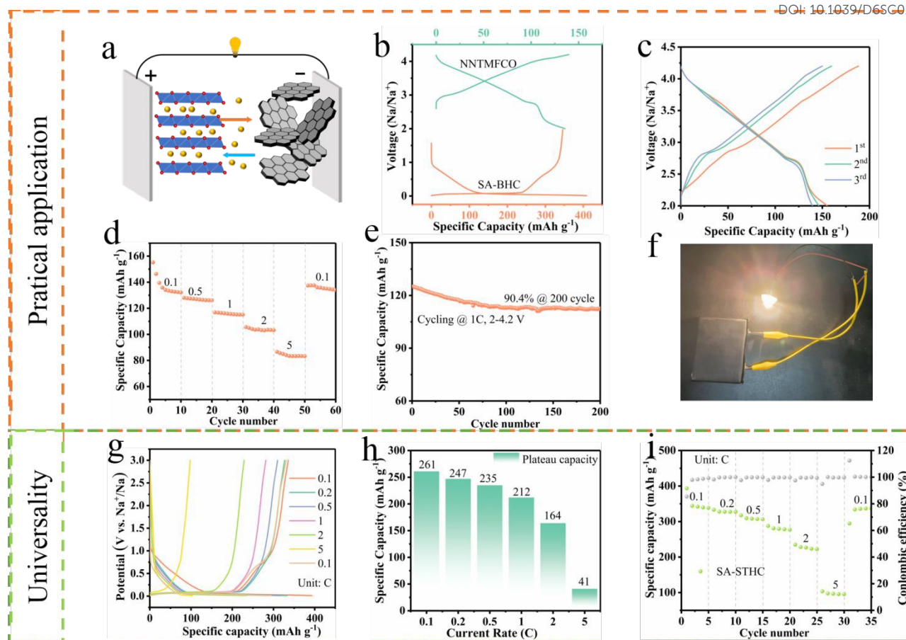
Fig. 7. (a) Schematic of the NNTMFCO||SA-BHC pouch-type full cell. (b) Capacity matching between the SA-BHC anode and NNTMFCO cathode. (c) Charge-discharge profiles of the NNTMFCO||SA-BHC pouch cell at 0.1C. (d) Rate capability from 0.1 to 5C. (e) Cycling performance at 1C. (f) Photograph of a yellow LED powered by the NNTMFCO||SA-BHC pouch cell. (g) GCD profiles of SA-STHC at 0.1-5C. (h) Plateau capacity of HC-Starch at 0.1-5C. (i) Rate performance of SA-STHC.
