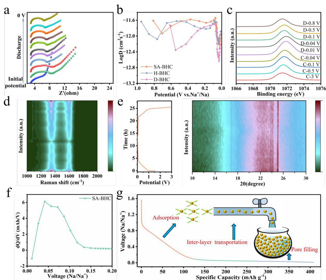
Fig. 4. (a) In situ EIS of the SA-BHC electrode during the discharge (sodiation) process. (b) GITT profiles of D-BHC, H-BHC, and SA-BHC. (c) Ex situ high-resolution Na 1s XPS spectra at selected states of charge. (d) In situ Raman spectra of the SA-BHC electrode during the first charge/discharge. (e) In situ XRD patterns of the SA-BHC electrode during the first charge/discharge. (f) Capacity differential ( dQ/dV ) curves of SA-BHC. (g) Schematic illustration of the sodium-storage stages in the SA-BHC anode.
