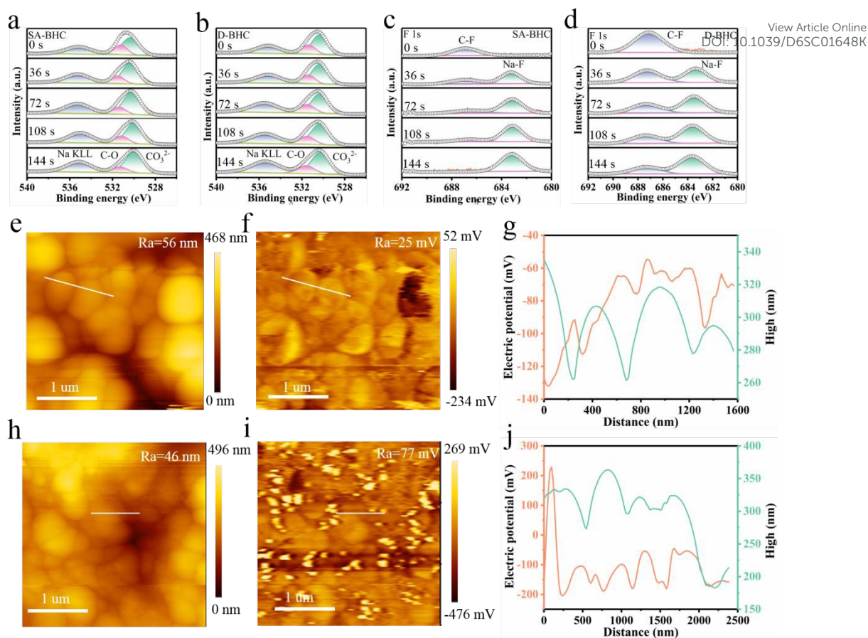
Fig. 6. Depth-resolved XPS spectra of cycled electrodes: (a,b) O 1s spectra of SA-BHC (a) and D-BHC (b); (c,d) F 1s spectra of SA-BHC (c) and D-BHC (d). KPFM characterization after 500 cycles: (e) topography of SA-BHC; (f) surface potential map; (g) correlated line profiles of surface potential and topography. (h) topography of D-BHC; (i) surface potential map; (j) correlated line profiles of surface potential and topography.
