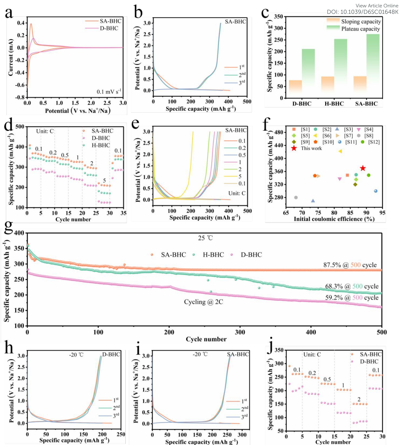
Fig. 3. (a) CV curves of D-BHC and SA-BHC at 0.1 mV s -1 . (b) GCD profiles of SA-BHC at 0.1C. (c) Comparison of slope and plateau capacities among D-BHC, H-BHC, and SA-BHC. (d) Rate performance from 0.1 to 5C. (e) GCD profiles of SA-BHC at rates from 0.1 to 5C. (f) Comparison of the reversible capacity and ICE of SA-BHC with those of reported bamboo-derived HC anodes for SIBs. (g) Long-term cycling performance at 2C. (h, i) GCD profiles of D-BHC and SA-BHC at 0.1C measured at room temperature and -20 °C. (j) Rate capability of D-BHC and SA-BHC at -20 °C.
