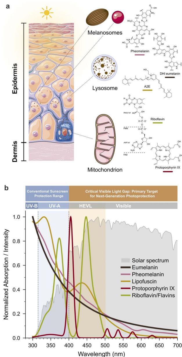
Fig. 7 Endogenous chromophores in human skin. (a) Schematic cross-section of the epidermis and upper dermis showing the subcellular localization of principal endogenous chromophores. A dendritic melanocyte at the basal layer synthesizes and transfers melanosomes to surrounding keratinocytes. Callouts highlight the three organelle compartments relevant to endogenous photosensitization, with representative chemical structures shown alongside. Eumelanin (dark brown, elongated granules) dissipates >99.9% of absorbed photon energy as heat through ultrafast internal conversion and is not an efficient photosensitizer. 150 Pheomelanin (reddish-brown granules) generates superoxide and \text{H}_2\text{O}_2 , functioning as a PI/PCI. Lipofuscin (yellow-green lysosomal aggregates) generates radicals that initiate lipid peroxidation chains, operating as a PI/PCI. PpIX (mitochondria) acts as a Type II/PS, and riboflavin/flavoproteins (mitochondria) function as membrane-associated PI/PCI (Box 1). (b) Spectral overlap between solar radiation and endogenous skin chromophores. Normalized absorption spectra of eumelanin (power-law model), 151 pheomelanin, 152 protoporphyrin IX, riboflavin, 153 and lipofuscin 154 are overlaid on the ASTM G173-03 AM1.5 global tilt solar irradiance spectrum (gray fill). Each absorption curve is normalized to its peak value within the displayed range. Conventional broad-
