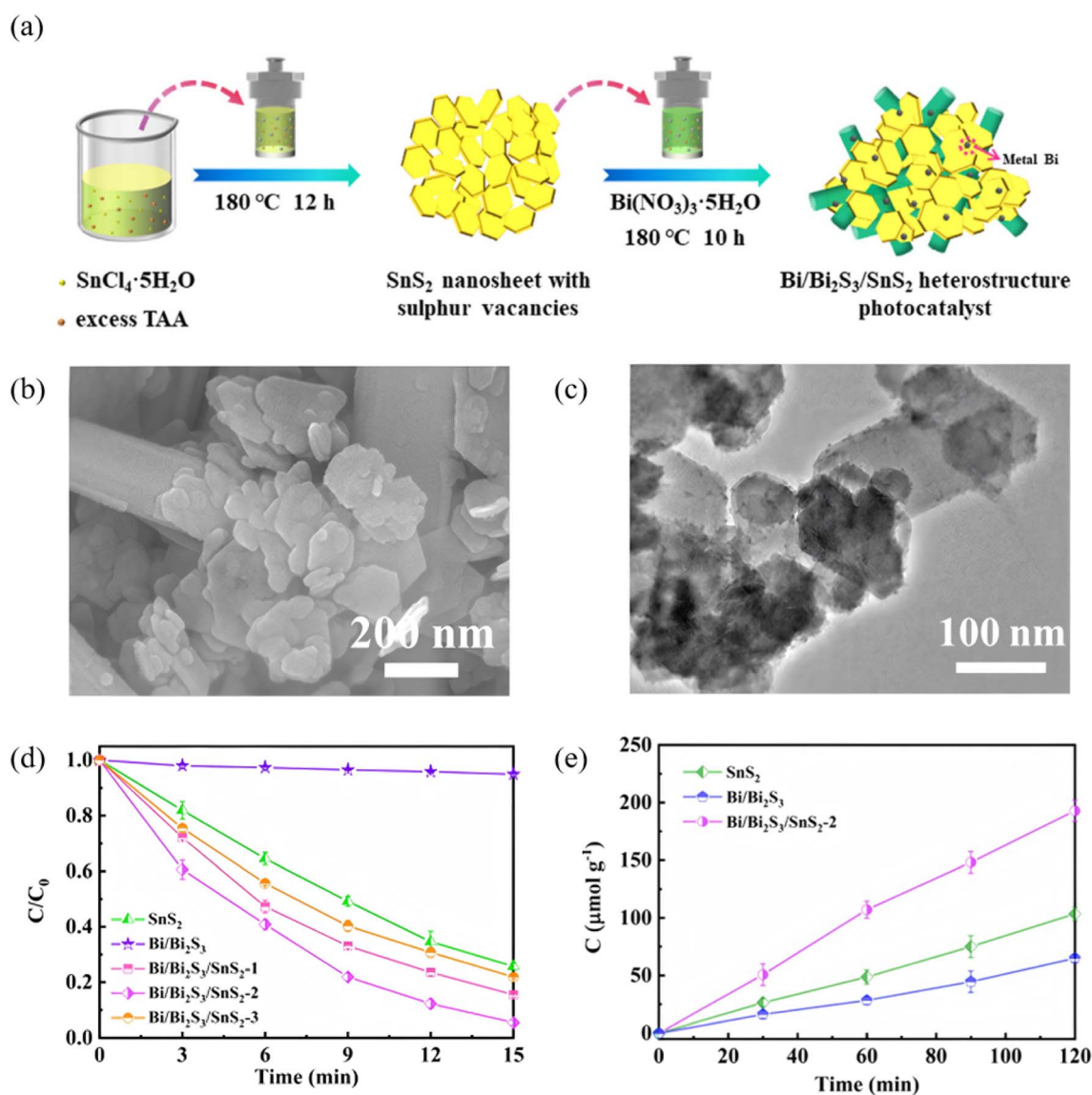
Fig. 22 (a) Diagram for the synthetic process of \text{Bi}/\text{Bi}_2\text{S}_3/\text{SnS}_2 heterostructure. (b) SEM and (c) TEM images of \text{Bi}/\text{Bi}_2\text{S}_3/\text{SnS}_2 -2. (d) Reduction curves of \text{Cr}(\text{VI}) by \text{SnS}_2 , \text{Bi}/\text{Bi}_2\text{S}_3 , and \text{Bi}/\text{Bi}_2\text{S}_3/\text{SnS}_2 . (e) Nitrogen fixation performance of \text{SnS}_2 , \text{Bi}/\text{Bi}_2\text{S}_3 , and \text{Bi}/\text{Bi}_2\text{S}_3/\text{SnS}_2 -2. 80 Copyright 2023, Chinese Society of Metals.
