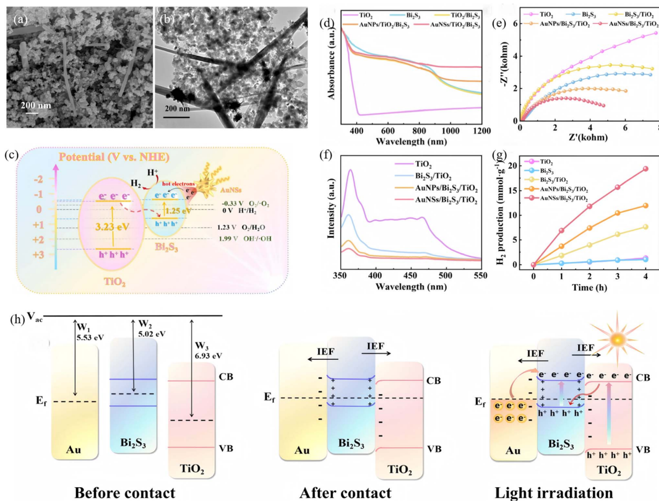
Fig. 17 (a) SEM and (b) TEM images of Au NSs/Bi 2 S 3 /TiO 2 . (c) Schematic representation of Schottky/S-scheme charge transfer mechanisms. (d) DRS spectra, (e) Electrochemical impedance spectroscopy, (f) PL spectra, (g) H 2 evolution performances of different samples, (h) Schottky/S-scheme heterojunction mechanisms including before contact, after contact, and under light irradiation. 72 Copyright 2025, Royal Society of Chemistry.
