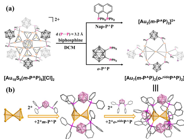
Fig. 3 (a) Structural transformation routes of \text{Au}_{18} reacting with bisphosphine ligands with similar P...P distances; (b) single crystal structure of \text{Au}_7 .
