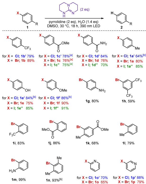
Fig. 2 Dehalogenation of chloro- (1') bromo- (1) and iodoarenes (1'). Reaction conditions: 1 (0.2 mmol), TBD (0.4 mmol), pyrrolidine (0.4 mmol), H 2 O (0.28 mmol), and 0.5 mL of DMSO. The solution was irradiated with a 390 nm LED and stirred at 30 °C for 18 h. All yields were determined by the average of two replicates using 1,3,5-trimethoxybenzene as an internal standard. [a]No pyrrolidine used. [b]Reaction time: 65 h.
