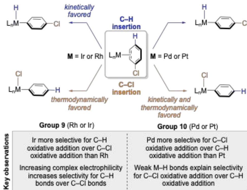
Scheme 1. Oxidative addition of the para -C–H bond and the C–Cl bond in chlorobenzene to Group 9 and Group 10 transition metal complexes and key observations from this work and previous experimental studies.
