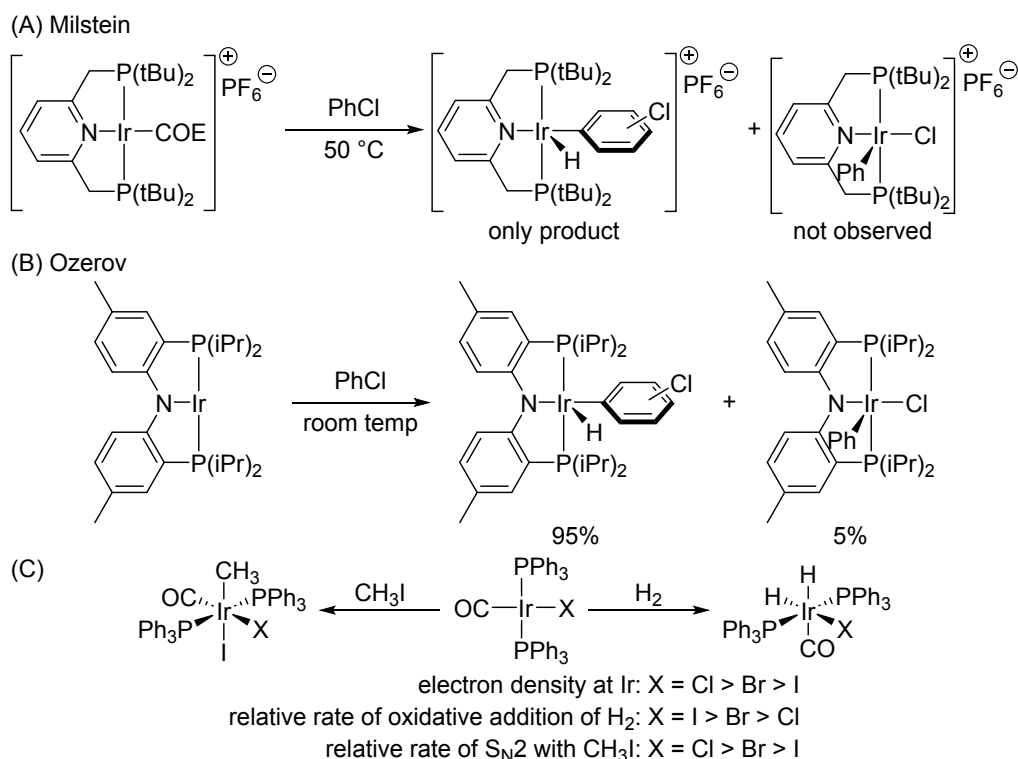
Figure 5. (A) Oxidative additions with a cationic (PNP)Ir complex (COE = cyclooctene); (B) oxidative additions with a neutral (PNP)Ir complex; (C) trends in relative rates of reactions with Vaska-type complexes.
