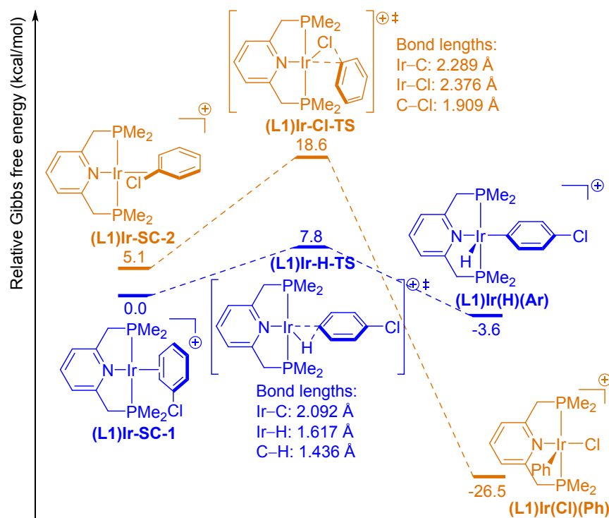
Figure 1. Free-energy diagram for the oxidative addition of the para -C–H bond (blue pathway) and the C–Cl bond (orange pathway) in PhCl to a cationic (L1)Ir(I) complex.
