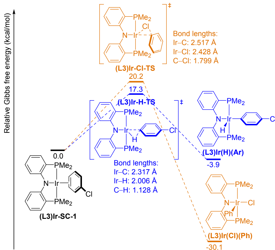
Figure 3. Free-energy diagram of the oxidative addition of the para -C–H bond (blue pathway) and the C–Cl bond (orange pathway) in PhCl to (L3)Ir(I) complexes.
