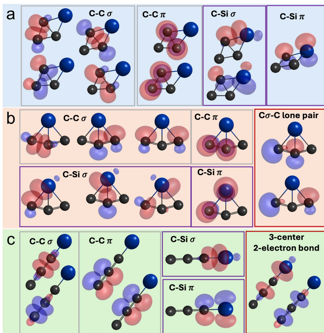
Fig. 7 Quasi-atomic orbital analysis (QUAO) of distinct \text{SiC}_3 isomers p1 (a), p2 (b), and p3 (c).
