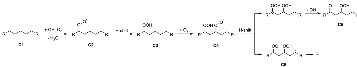
Fig. 1 Key steps in autoxidation of an example VOC. The compound C1 first reacts with OH radical and O 2 to form a peroxy radical (C2), which undergoes an H-shift forming a hydroperoxide functionality and a radical center on the carbon from which the H atom was abstracted, also known as a hydroperoxyalkyl radical or QOOH (C3). Subsequent addition of O 2 forms a hydroperoxy RO 2 (C4), which can undergo further H-shifts. The reaction sequence can either be terminated by abstracting the H atom \alpha to the hydroperoxide group and losing a OH radical to form a ketohydroperoxide (C5), or continue by abstracting a H atom from an unsubstituted carbon to form a new, more oxidized QOOH (C6).
