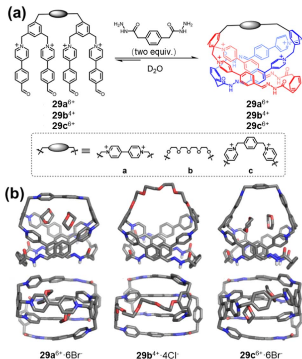
Fig. 33 (a) Synthesis and chemical structures of the pretzelanes 29a 6+ , 29b 4+ , and 29c 6+ ; (b) side and top views of the solid-state structure of 29a 6+ ·6Br - , 29b 4+ ·4Cl - , and 29c 6+ ·6Br - . Reproduced from ref. 130. Copyright 2025 American Chemical Society.
