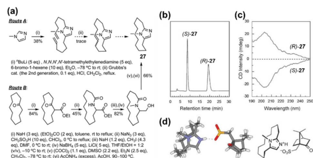
Fig. 31 (a) Synthesis of the cyclophane-type imidazole 27; (b) chiral HPLC trace of 27; (c) CD spectra of (R)- and (S)- 27 in H 2 O; (d) X-ray crystal structure of the salt of (S)- 27 with (+)-10-camphorsulfonic acid. Reproduced from ref. 125. Copyright 2009 Royal Society of Chemistry.
