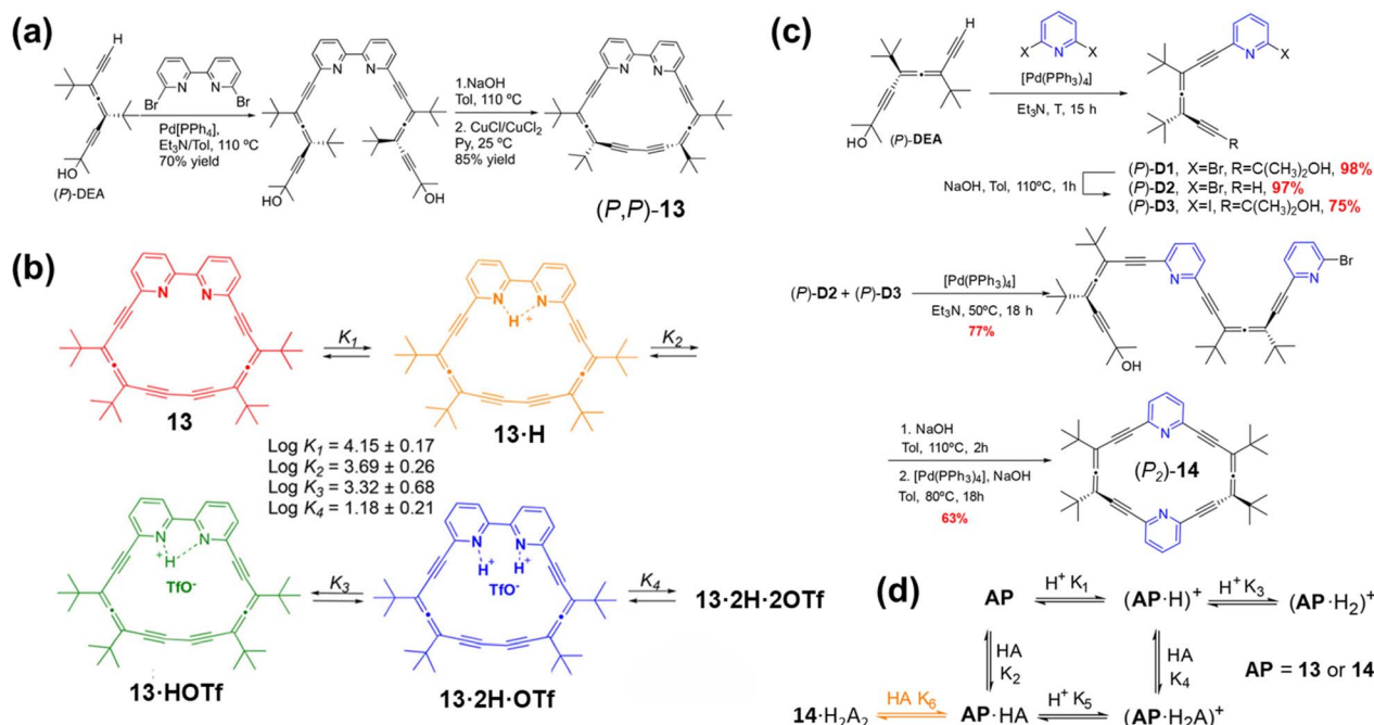
Fig. 17 (a) Synthesis of allenophanes 13 ; (b) proposed scheme for titration process for (P,P)-13 with TfOH in CH_3CN ; Reproduced from ref. 97. Copyright 2019, American Chemical Society. (c) Synthesis of allenophanes 14 ; (d) titration scheme for allenophanes 13 and 14 with oxoacids. The equilibrium in orange is only relevant for compound 14 . (AP = Allenophane). Reproduced from ref. 98. Copyright 2023, Royal Society of Chemistry.
