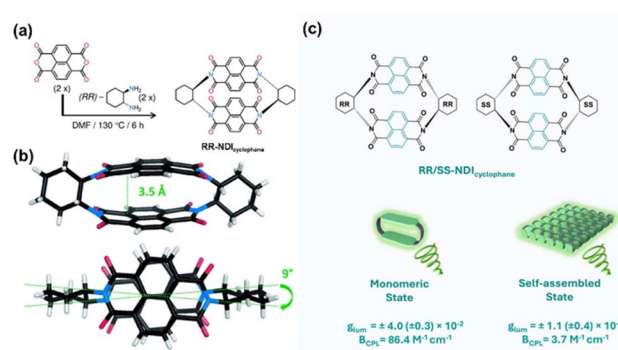
Fig. 14 (a) Synthesis of RR-NDI cyclophane ; (b) solid-state structure of RR-NDI cyclophane in both top and side views; Reproduced from ref. 85. Copyright 2014 WILEY-VCH. (c) Schematic representation of key CPL parameters, including g_{\text{Lum}} and B_{\text{CPL}} for the monomeric and self-assembled states of RR/SS-NDI cyclophane . Reproduced from ref. 86. Copyright 2025 WILEY-VCH.
