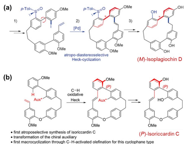
Fig. 20 Atropo-diastereoselective Heck coupling for the synthesis of enantiopure (a) Isoplagiochin D Reproduced from ref. 103. Copyright 2018 Wiley-VCH and (b) Isoriccardin C. Reproduced from ref. 104. Copyright 2021 Wiley-VCH.
