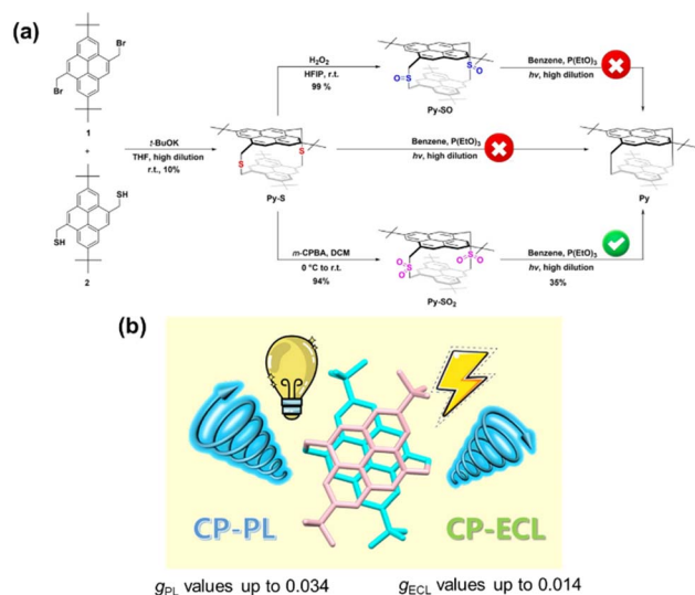
Fig. 50 (a) Synthesis of planar chiral pyrenophanes Py-S , Py-SO , Py-SO 2 , and Py ; (b) these pyrenophanes exhibit stable and intense CP-PL and CP-ECL properties. Reproduced from ref. 152. Copyright 2025 Wiley-VCH.
