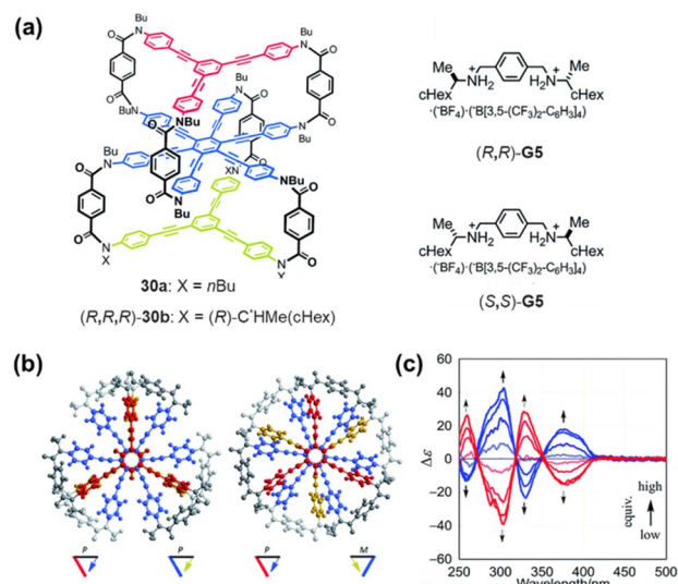
Fig. 36 (a) Structures of 30a, ( R,R,R )-30b, and chiral guest molecules ( R,R )/( S,S )-G5; (b) computationally optimized predominant conformation of 30a' ( X = \text{Me} ); (c) CD spectra of 30a' ( 7.1 \times 10^{-5} \text{ M} ) in the presence of a chiral guest [3, 6, 8 and 12 equiv. of ( S,S )-G5 (red lines) or ( R,R )-G5 (blue lines)]. Reproduced from ref. 137. Copyright 2018, Royal Society of Chemistry.
