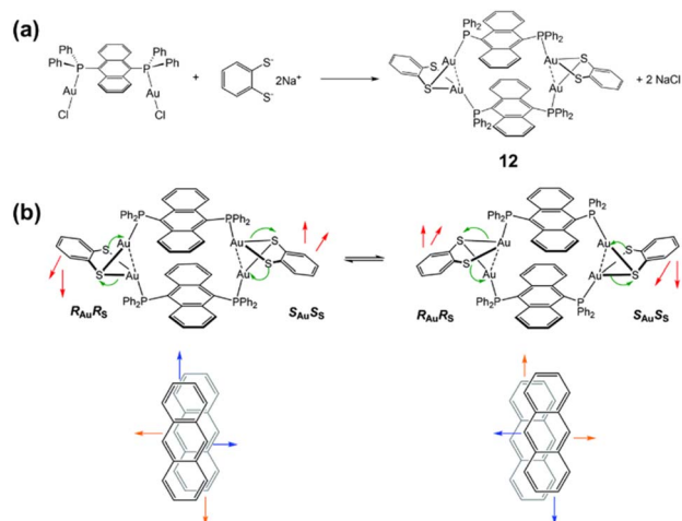
Fig. 16 (a) Structure of the tetranuclear gold(i) cyclophane 12; (b) schematic representation of the intramolecular dynamic exchange of Au–S bonds. Reproduced from ref. 88. Copyright 2021 Royal Society of Chemistry.
