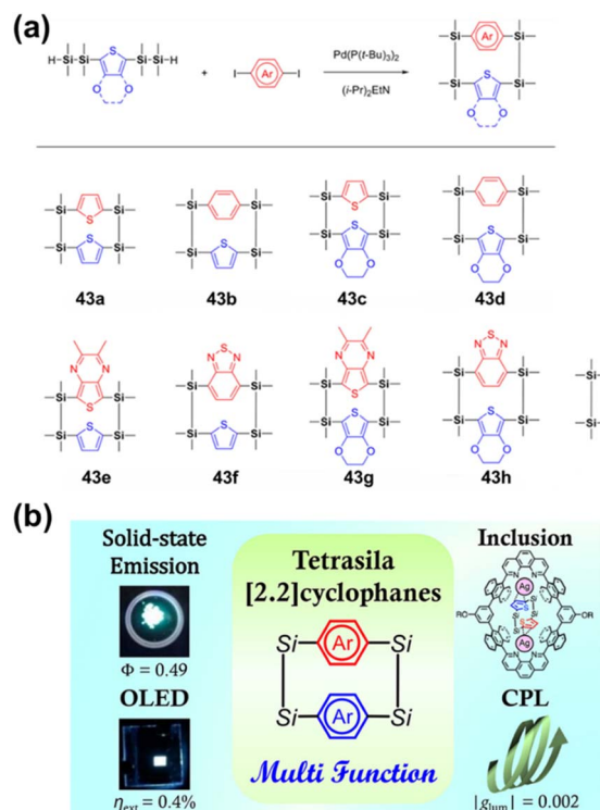
Fig. 51 (a) Synthesis of planar chiral tetrasila[2.2]cyclophanes 43a–i ; (b) schematic illustration of the luminescence properties of tetrasila[2.2]cyclophanes, highlighting their solid-state emission and CPL characteristics with potential applications in OLED. Reproduced from ref. 153. Copyright 2017 American Chemical Society.
