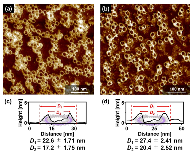
Fig. 5 (a, b) AFM images of SP ring obtained by sonicating a SP hel solution of 1 ( c = 50 \mu\text{M} ) in (a) MCH and (b) MCH including 0.7% (v/v) THF. (c, d) AFM cross-sectional analyses of representative SP ring
