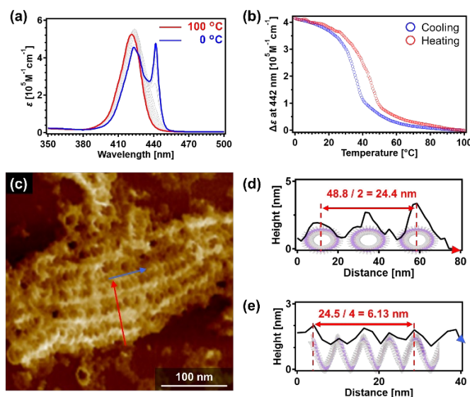
Fig. 4 (a) UV/Vis absorption spectra of 1 in MCH including 0.7% (v/v) of THF ( c = 54 \mu\text{M} ) upon cooling from 100 °C (red line) to 0 °C (blue line) at a rate of 1 °C min -1 . The intermediate spectra were measured every 5 °C. (b) Cooling (blue plots) and heating (red plots) profiles obtained by plotting change in absorbance at 442 nm as a function of temperature. (c) AFM image of the resulting assemblies. (d, e) AFM cross-sectional analyses along the (d) red and (e) blue arrows in (c), respectively.
