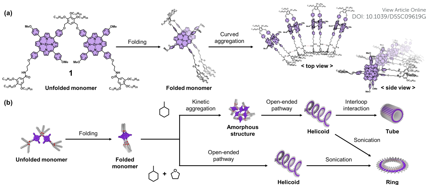
Fig. 1 (a) Molecular structure of 1 . (b) Schematic representation of its self-assembly process to form helicoid, tube and ring.
