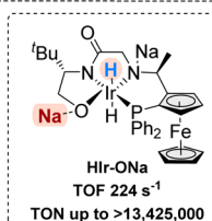
(C) This work: Ir/Huaphos catalyzed asymmetric hydrogenation of N -aryl indole ketones (and aldehydes)
