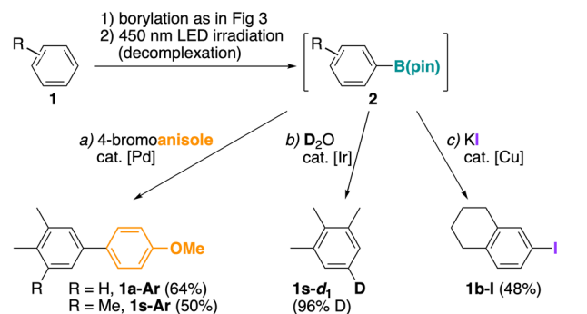
Fig. 4 Borylation of 1 , followed by derivatization of 2 . (a) 4-Bromoanisole (1.2 equiv.), [\text{Pd}_2(\text{dba})_3]\cdot\text{CHCl}_3 (2.5 mol%), XPhos (5 mol%), \text{K}_3\text{PO}_4 (3 equiv.); THF/ \text{H}_2\text{O} (10 : 1), 80\text{ }^\circ\text{C} , 12 h. (b) \text{D}_2\text{O} (10 equiv.), [\text{Ir}(\text{cod})(\text{OMe})_2] (2 mol%); THF, 80\text{ }^\circ\text{C} , 3 h. (c) KI (3 equiv.), [Cu] (10 mol%), Phen (20 mol%); MeOH/ \text{H}_2\text{O} (4 : 1), 80\text{ }^\circ\text{C} , 12 h.
