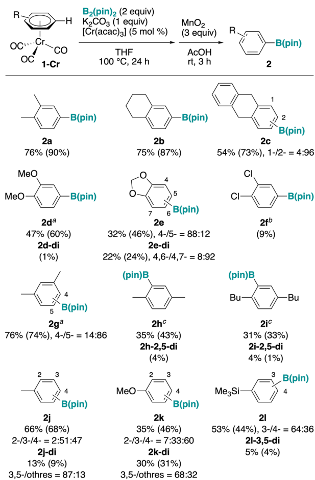
Fig. 2 Preliminary investigation of a model reaction, the borylation of arene chromium complexes 1-Cr . The yields were determined by isolation; the yields in parentheses were determined by using 1 H NMR or GC in the presence of an internal standard. See the SI for details. a Reaction time was 68 h. b Reaction time was 17 h. c Reaction time was 4 days.
