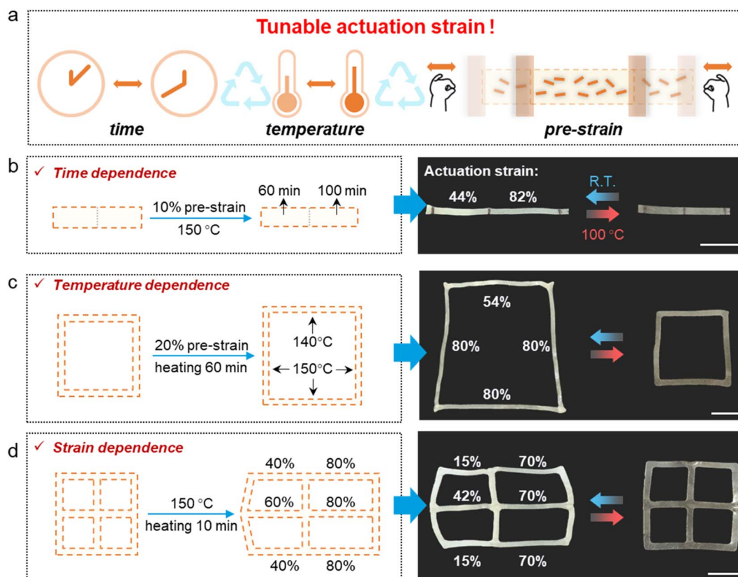
Fig. 8 (a) The actuation strain of xLCEs is tunable by adjusting the programming pre-strain, temperature, and time. (b–d) Spatially actuated strains were achieved by locally tuning the degree of topology rearrangement through modulation of (b) programming time, (c) programming temperature, and (d) applied pre-strain. Scale bars: 1 cm.
