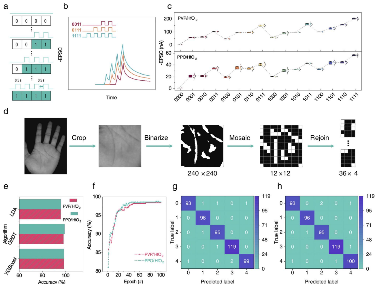
Fig. 4 (a) Device response to a 4-bit light stimulus, where “1” and “0” represent 365 nm light and dark conditions, respectively, with a light pulse width of 0.5 s and pulse interval of 0.5 s. (b) I - t light response curves for three representative inputs “0011”, “0111” and “1111”. (c) PVP/HfO 2 -based and PPO/HfO 2 -based devices in response to 4-bit light stimulus. (d) Pre-processing of the palmprint images, including cropping, binarizing, mosaic and rejoining. (e) The accuracy of three different algorithms based on PVP/HfO 2 -based and PPO/HfO 2 -based devices. (f) Evolution of accuracy based on PVP/HfO 2 -based and PPO/HfO 2 -based devices. (g) The confusion matrix of the PVP/HfO 2 -based device shows accurate classification and misclassification. (h) The confusion matrix of the PPO/HfO 2 -based device shows accurate classification and misclassification.
