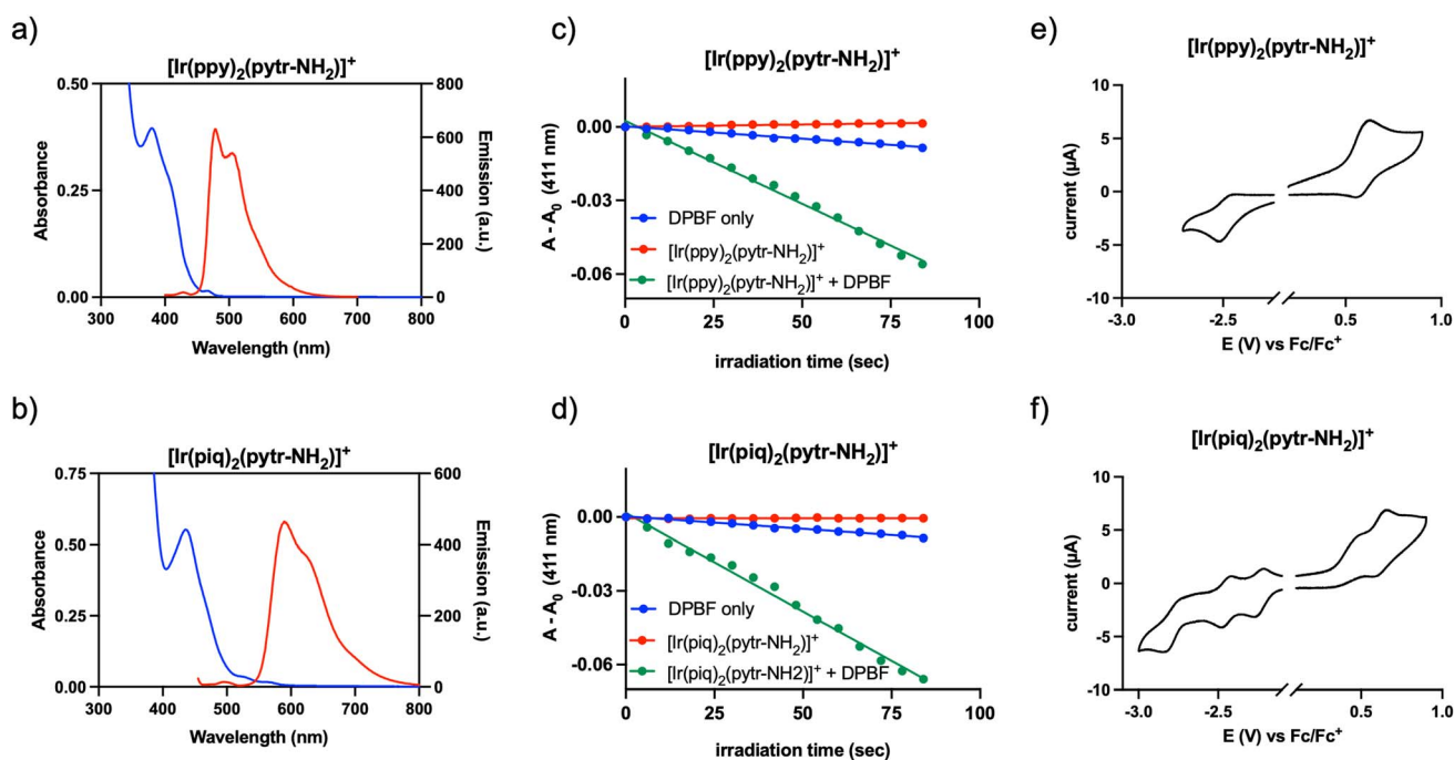
Fig. 2 (a) and (b) MLCT absorbance (blue) and emission (red) spectra of [Ir(ppy) 2 (pytr-NH 2 )] + and [Ir(piq) 2 (pytr-NH 2 )] + in acetonitrile. (c) and (d) plot of A-A_0 at 411 nm for DPBF (10 μM, blue) [Ir(ppy) 2 (pytr-NH 2 )] + or [Ir(piq) 2 (pytr-NH 2 )] + only (red), and DPBF with [Ir(ppy) 2 (pytr-NH 2 )] + or [Ir(piq) 2 (pytr-NH 2 )] + (green). (e) and (f) Cyclic voltammograms of [Ir(ppy) 2 (pytr-NH 2 )] + and [Ir(piq) 2 (pytr-NH 2 )] + , in acetonitrile, 200 mV s -1 , potentials quoted versus ferrocenium/ferrocene.
