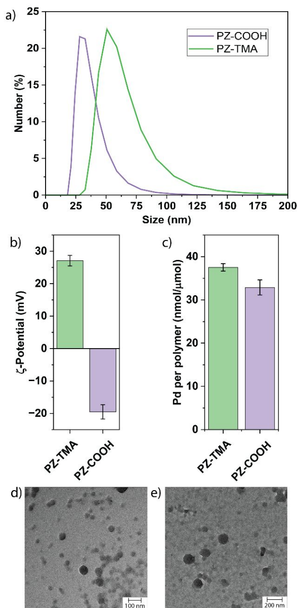
Figure 2. a) Size distribution measured by dynamic light scattering (DLS); b) \zeta -potential of respective PZs; c) quantification of encapsulated Pd 106 measured by inductively coupled plasma mass spectrometry (ICP); TEM images of d) PZ-TMA and e) PZ-COOH.
