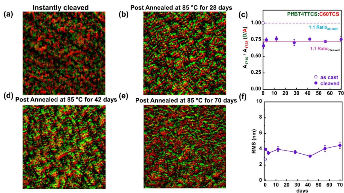
Figure 4. Stability measurement of the active layer (PffBT-4T-TCS:C60TCS=1:1) under continuous annealing at 85 °C: a) Overlay image of the cleaved active layer immediately after thermal cleavage; b) Overlay image of the cleaved active layer after annealing at 85 °C for 28 days; c) Evolution of local chemical compositions for as-cast and cleaved active layer as a function of annealing time; d) Overlay image of the cleaved active layer after 42 days of annealing at 85 °C; e) Overlay image of the cleaved active layer after 70 days of annealing at 85 °C; f) surface roughness as a function of annealing time. In all overlay images, green and red regions represent donor and acceptor, respectively.
