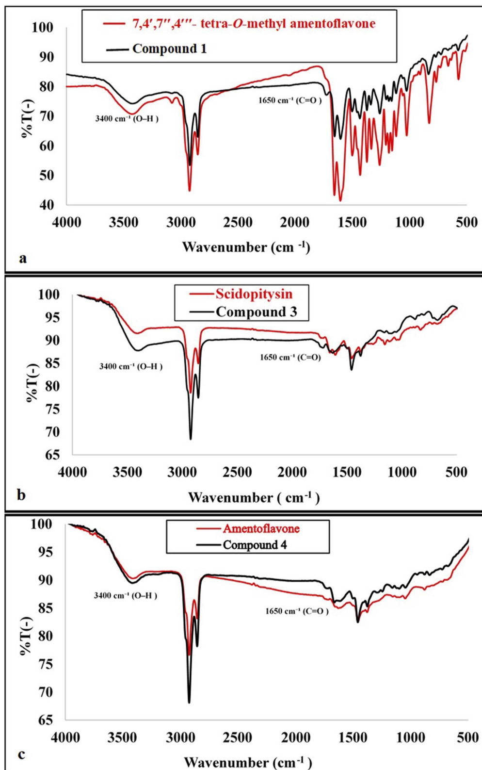
Fig. 4 Superimposed FTIR spectra of the isolated biflavonoids and their authentic standards: (a) 7,4',7'',4'''-tetra-O-methyl amentoflavone (compound 1), (b) scidopitysin (compound 3), (c) amentoflavone (compound 4) showing characteristic absorption bands and strong spectral overlap, particularly in the fingerprint region.
