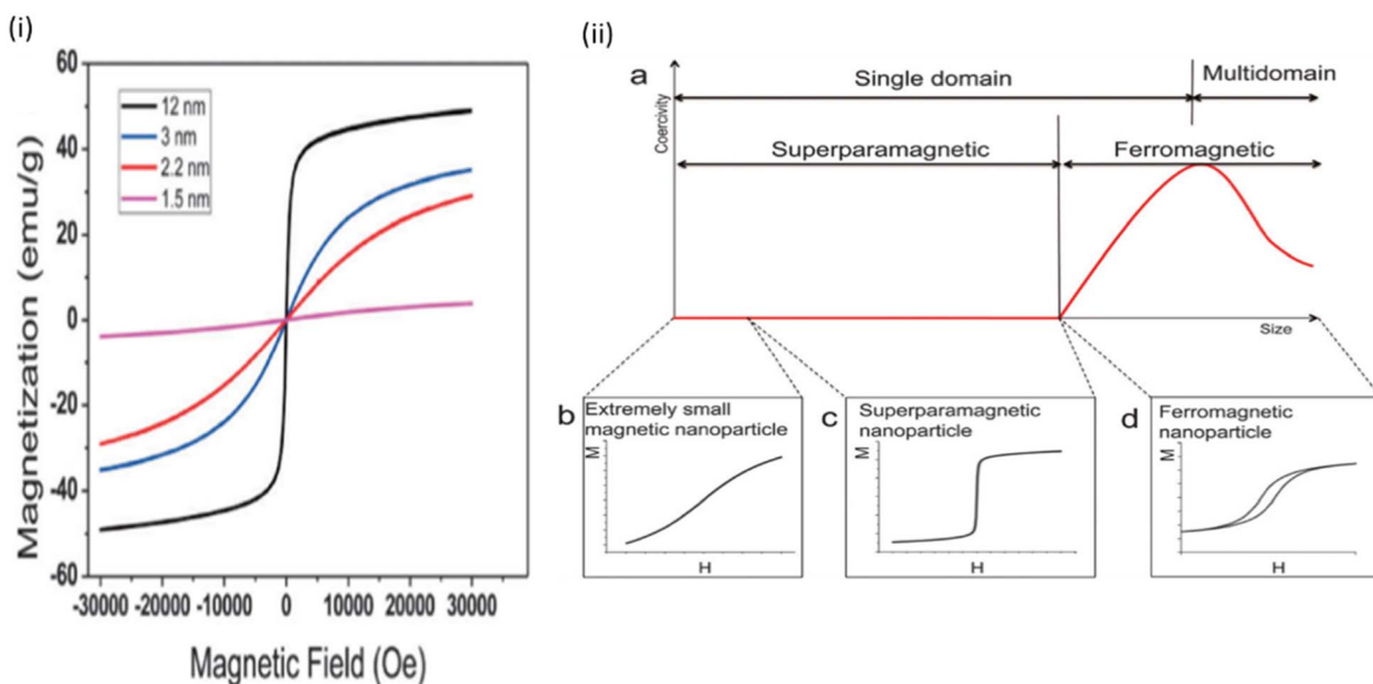
Fig. 12 (i) Field-dependent magnetization ( M – H ) curves of IONPs with diameters of 1.5 nm (pink), 2.2 nm (red), 3 nm (blue), and 12 nm (black) at 300 K. (ii) (a) Variation of coercivity with nanoparticle size. (b) M – H curve of extremely small magnetic nanoparticles. (c) M – H curve of superparamagnetic nanoparticles. (d) M – H curve of ferromagnetic nanoparticles.
