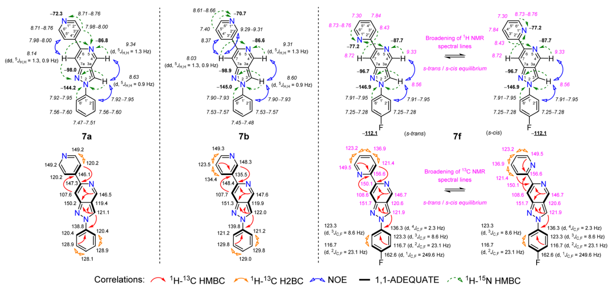
Fig. 2 Relevant 1 H– 13 C HMBC, 1 H– 13 C H2BC, 1 H– 15 N HMBC, 1,1-ADEQUATE, and 1 H– 1 H NOESY correlations, as well as 1 H NMR (italic), 13 C NMR, 15 N NMR (bold), and 19 F NMR (bold, underlined) chemical shifts of compounds 7a , 7b , and 7f (CDCl 3 ).
