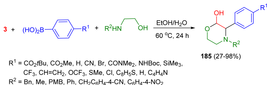
Scheme 74 Synthesis of 2-hydroxy-3-arylmorpholines 185 using the Petasis borono-Mannich reaction.
