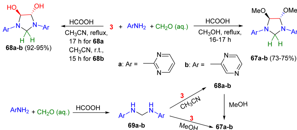
Scheme 22 Synthesis of the imidazolidine derivatives 67 and 68.
