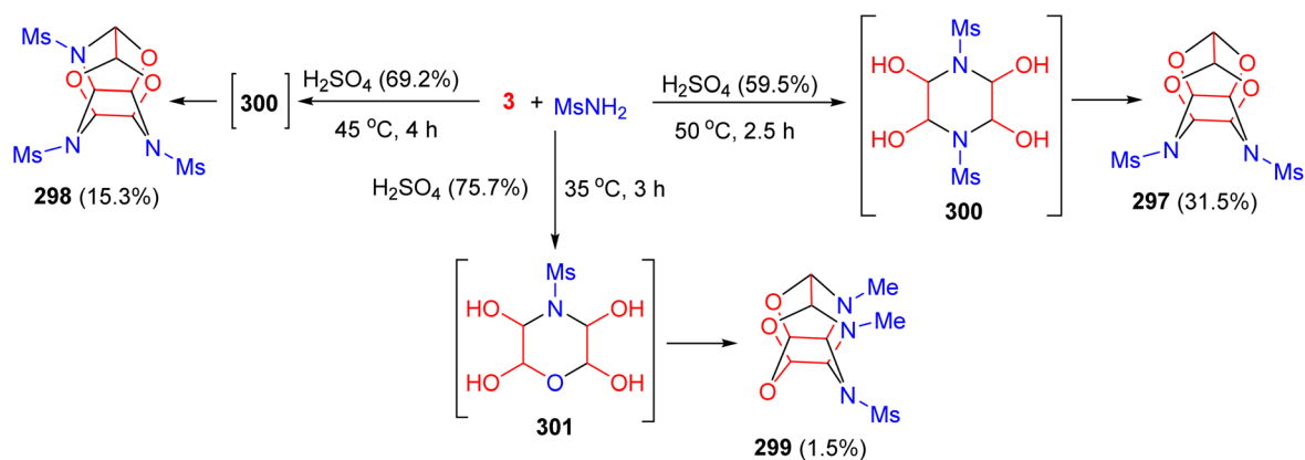
Scheme 120 Sulfuric acid catalyzed synthesis of oxazaisowurtzitane 297–299 .
