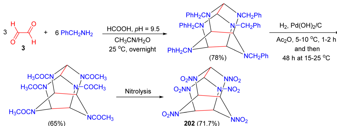
Scheme 84 Formic acid catalyzed synthesis of hexanitrohexaazaisowurtzitane (HNIW) ( 202 ).
