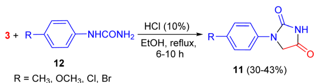
Scheme 4 HCl-catalyzed synthesis of 1-aryl substituted hydantoins 11 .
