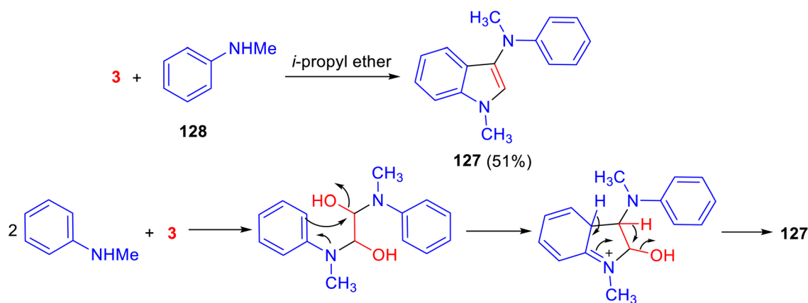
Scheme 51 Synthesis of l-methyl-3-(methylphenylamino)indole ( 127 ).
