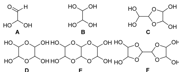
Fig. 1 Different structures of aqueous glyoxal (A–F).
