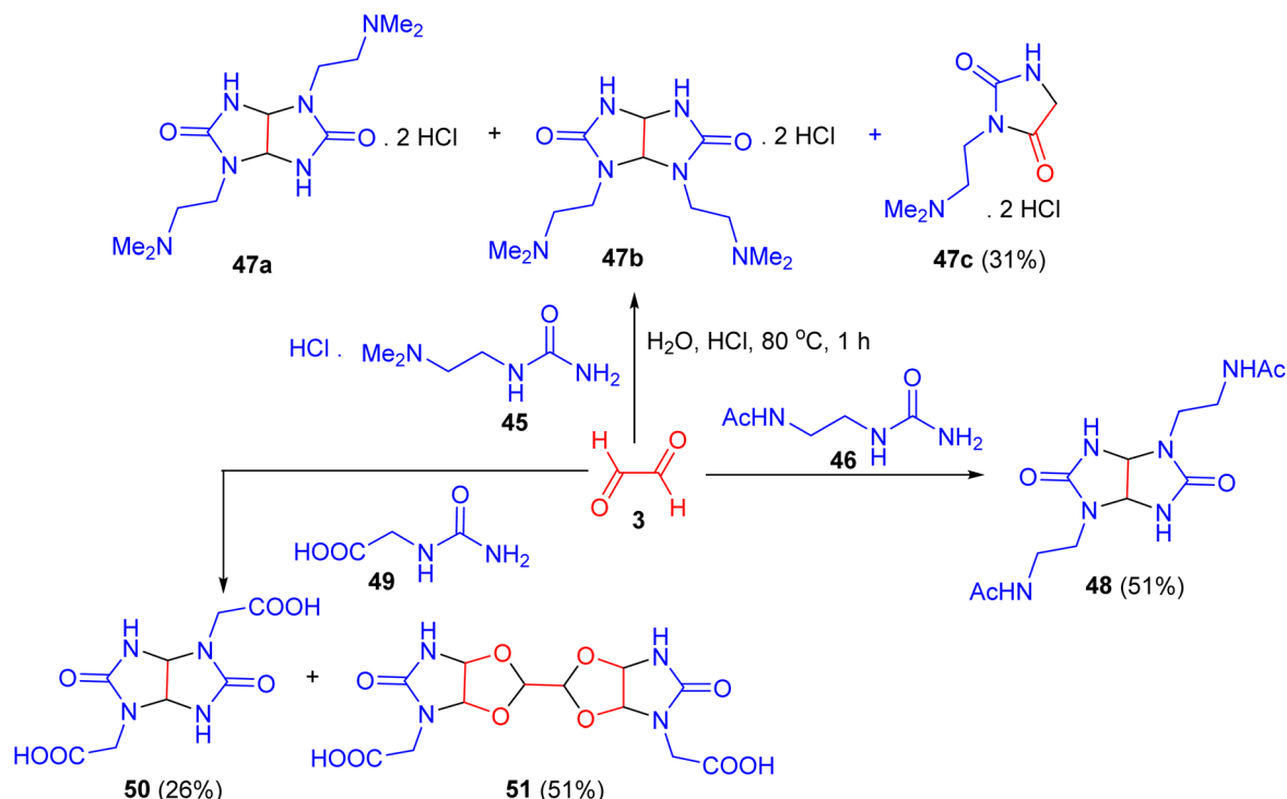
Scheme 16 Regioselective synthesis of glycurils 47, 48 and 50.
