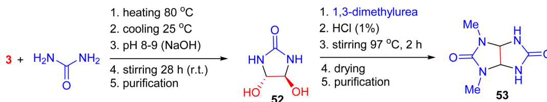
Scheme 17 Synthesis of trans -4,5-dihydroxy-2-imidazolidinone 52 and 2,4-dimethylglycuril 53.
