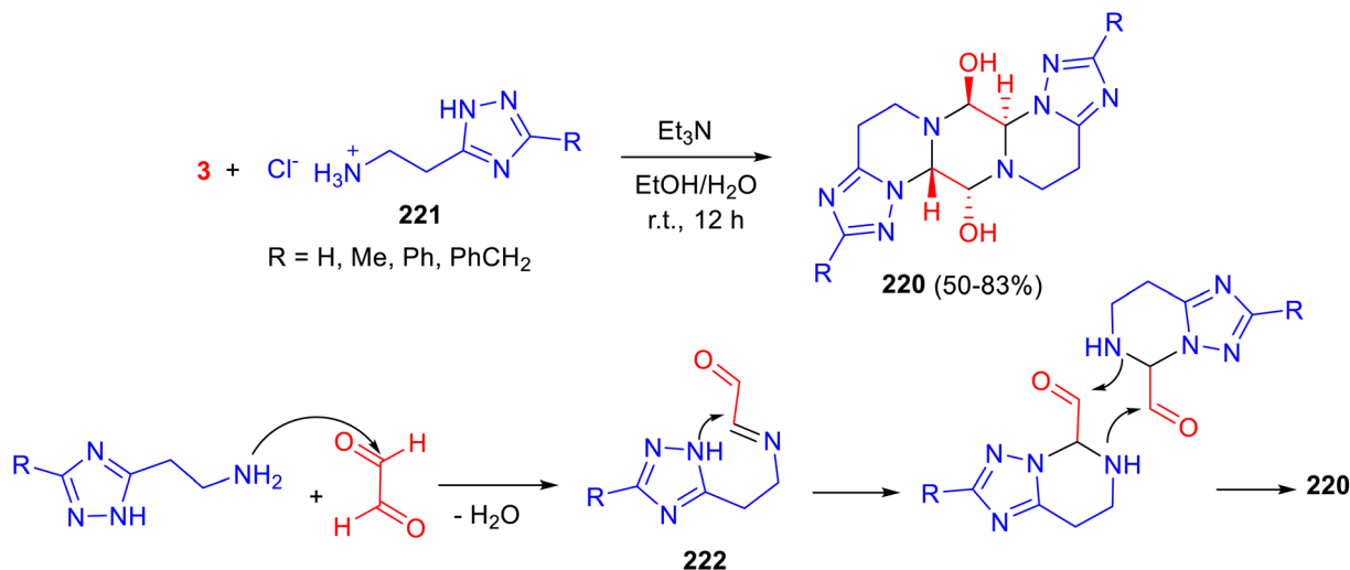
Scheme 94 Preparation of pentacyclic heterocycles 220.
