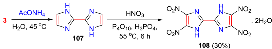
Scheme 41 Synthesis of the biimidazole derivatives 107 and 108 .
