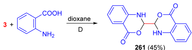
Scheme 109 Synthesis of 2,2'-bis(1,2-dihydro-4-oxo-3,1-benzoxazine) (261).
