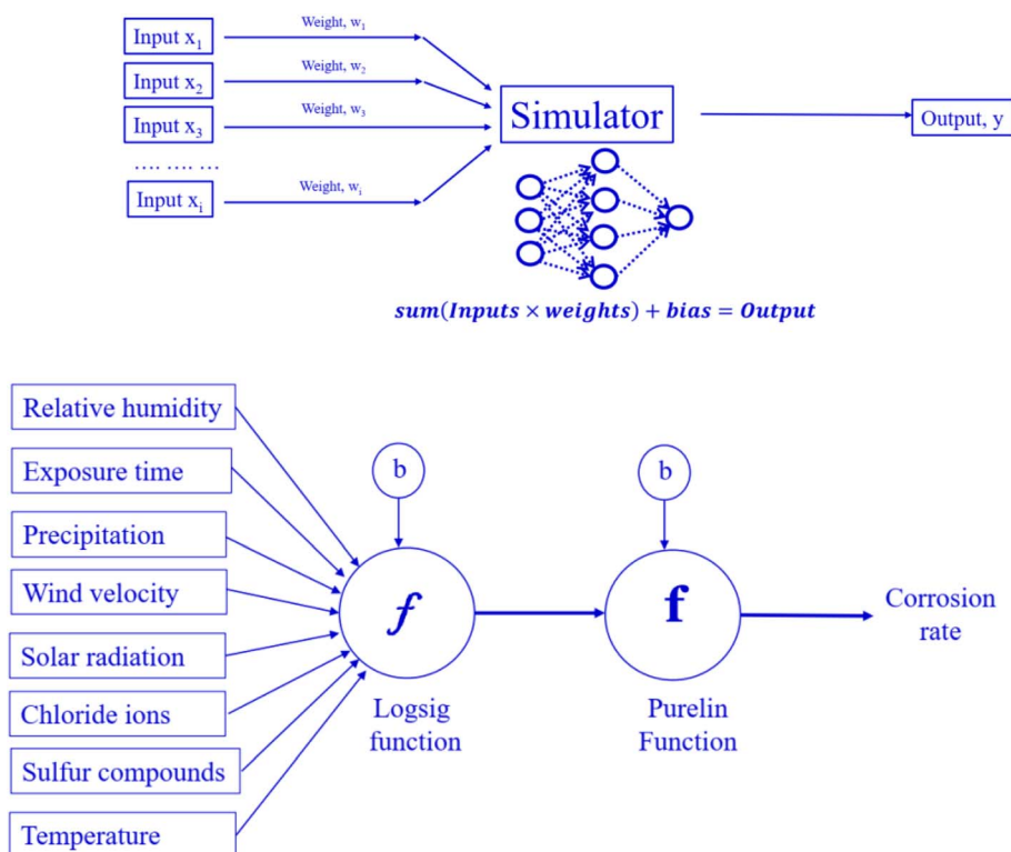
Fig. 31 Artificial Neural Network (ANN) model with linear and sigmoidal functions to predict environmental parameters.
