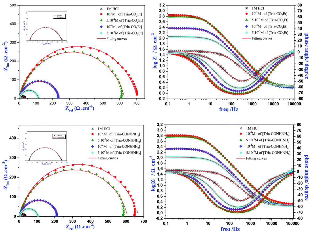
Fig. 19 Nyquist and Bode plots for mild steel in 1.0 M HCl with and without various [Tria- \text{CO}_2\text{Et} ] and [Tria- \text{CONHNH}_2 ] concentrations, reproduced from ref. 56 with permission from [RSC] [RSC Adv., 2021, 11, 4147–4162] copyright 2021.
