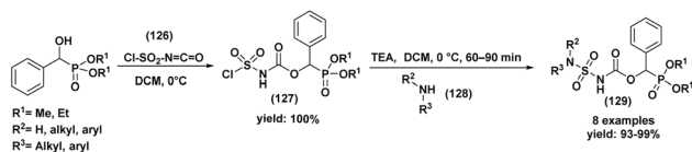
Scheme 32 Synthesis of sulfamidocarbonyloxyphosphonates starting from \alpha -hydroxyphosphonates.
