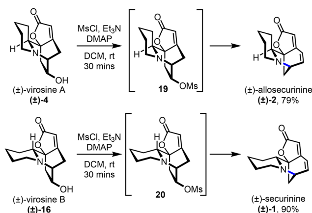
Scheme 3 Synthesis of ( \pm )-allosecurinine and ( \pm )-securinine.
