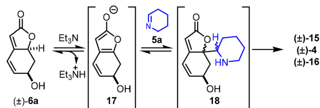
Scheme 2 Outline mechanism for the formal [4 + 2] cycloaddition to form ( \pm )-15, ( \pm )-4 and ( \pm )-16.
