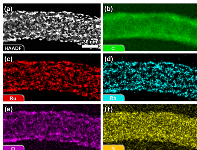
Fig. 24 (a) High angle annular dark field (HAADF) image of the RuRhCNT hybrid and associated EDS mapping for (b) carbon; (c) ruthenium; (d) rhodium; (e) oxygen; and (f) nitrogen.
