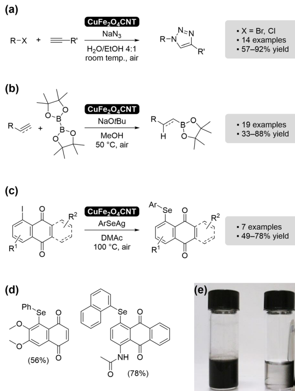
Fig. 26 Transformations using CuFe 2 O 4 CNT as a catalyst: (a) 1,3-dipolar cycloaddition of alkynes with in situ generated azides; (b) borylation of alkenes and alkynes; and (c) A-ring selenation of naphthoquinones. (d) Examples of selenated quinone products. (e) Application of a permanent magnet for easy recovery of the catalyst.
