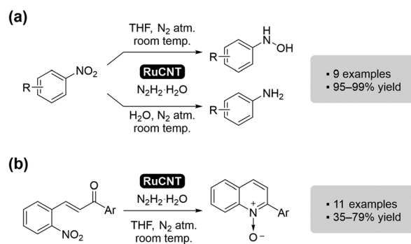
Fig. 20 Hydrazine-mediated processes using RuCNTs: (a) hydrogenation of nitroarenes and (b) conversion of 2-nitrochalcones to quinoline N -oxides.
