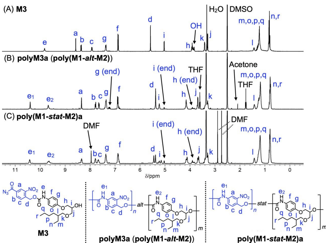
Figure 5. ^1\text{H} NMR spectra of (A) M3 ; (B) polyM3a (poly(M1- alt -M2)) ; (C) poly(M1- stat -M2)a (400 MHz, 298 K, \text{DMSO-d}_6 ).
