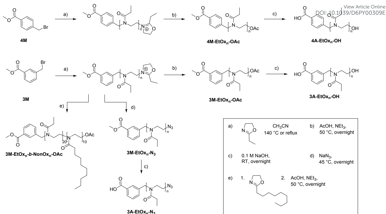
Scheme 1: Schematic representation of the CROP of 2-oxazolines initiated by 4M and 3M (a) including chain extensions (e), termination reactions (b, d) and post-polymerization deprotection (c) used to obtain POx with \alpha -terminal carboxylic acid moieties.
