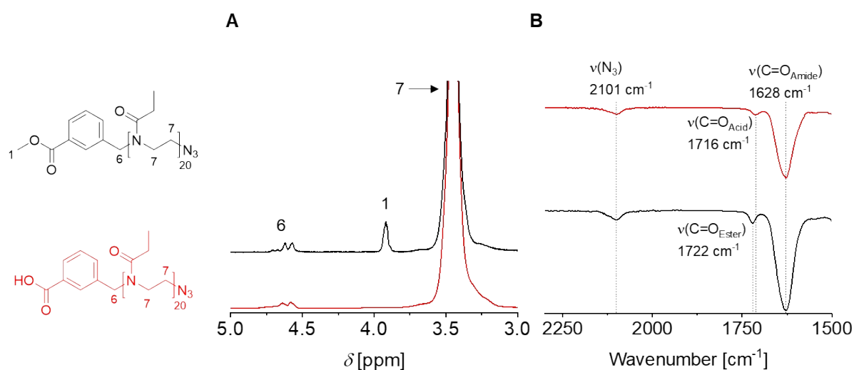
Figure 5: Spectroscopic confirmation of end groups in the heterotelechelic 3M-EtOx 20 -N 3 (black) and 3A-EtOx 20 -N 3 (red). A: Overlay of 1 H NMR spectra (CDCl 3 , 300 MHz). B: Overlay of IR spectra with assignment of characteristic vibrational bands. Full spectra are shown in the supporting information.
