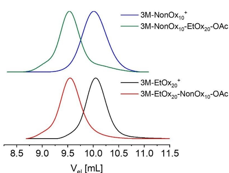
Figure 4. SEC elugrams (RI detection) of 3M\text{-NonOx}_{10}\text{-}b\text{-EtOx}_{20}\text{-OAc} and 3M\text{-EtOx}_{20}\text{-}b\text{-NonOx}_{10}\text{-OAc} as well as of the corresponding first blocks 3M\text{-NonOx}_{10}^+ and 3M\text{-EtOx}_{20}^+ before the addition of the second monomer.
