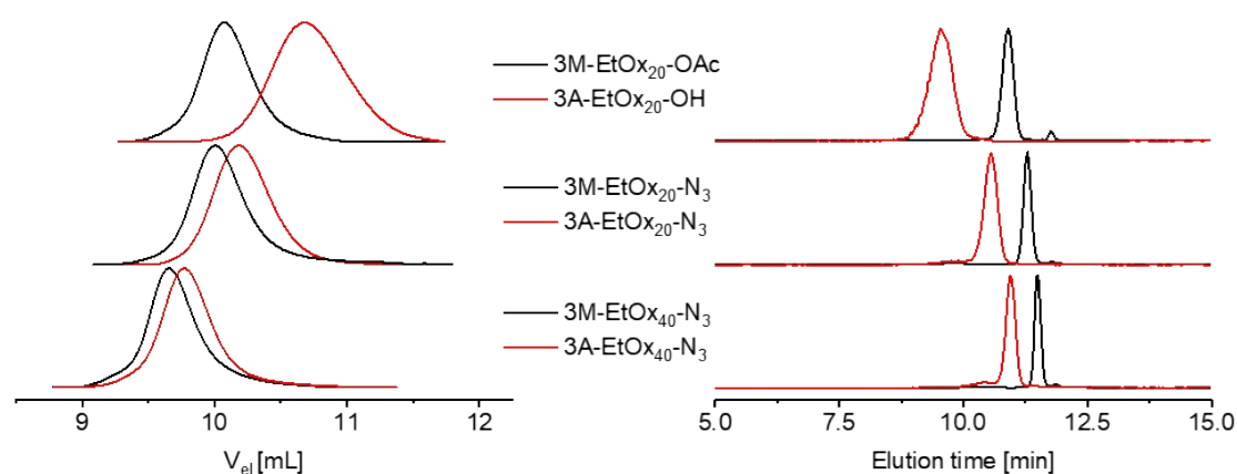
Figure 6: Chromatographic analysis of protected and deprotected PEtOx heterotelechelic oligomers obtained by initiation of CROP with 3M . Left: SEC (RID). Right: HPLC (RP18 Chromolith column, water/acetonitrile gradient with 0.1% formic acid, ELSD).
