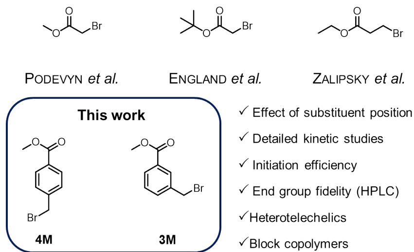
Figure 1: Schematic representation of initiators used in previous works and in this study.
