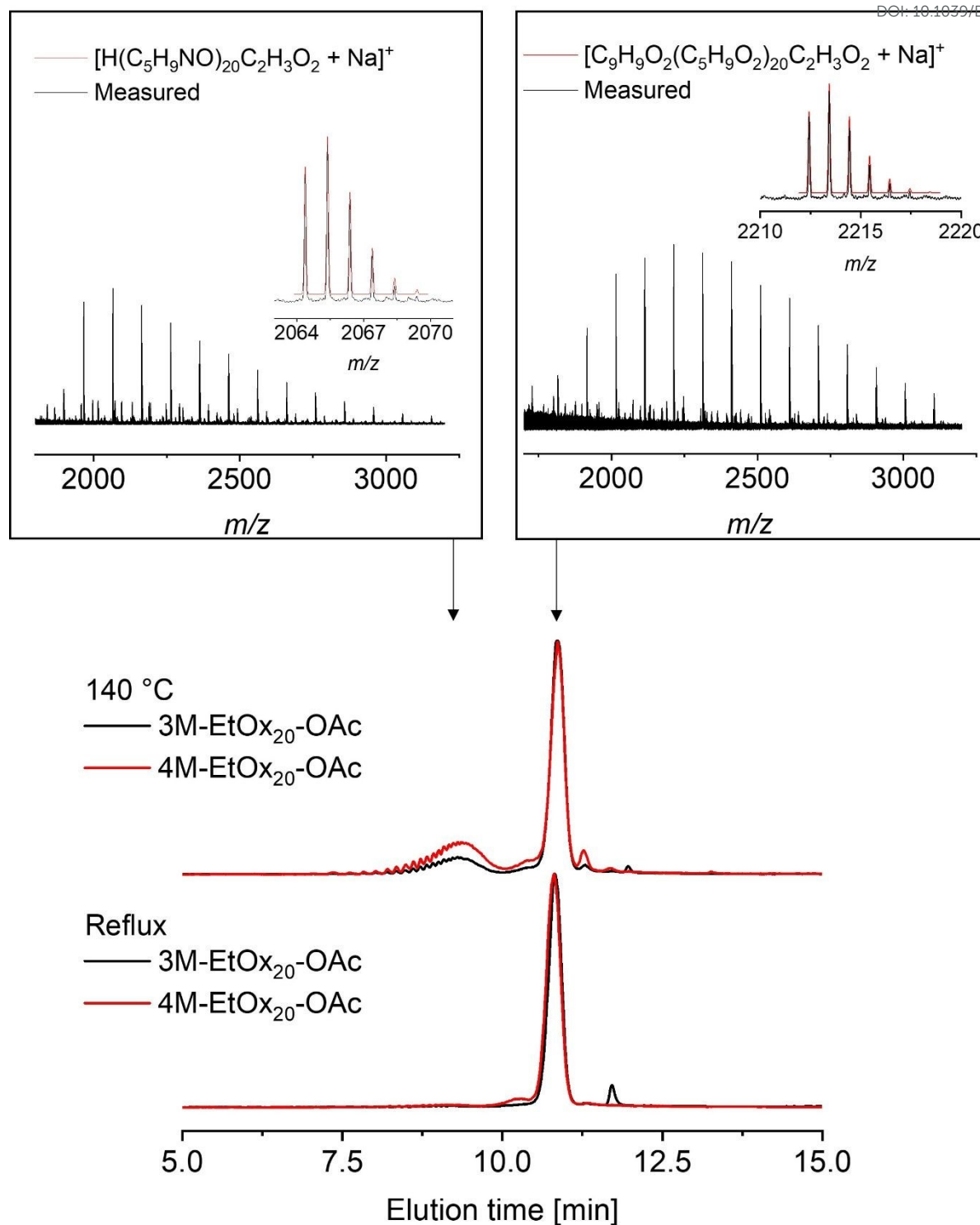
Figure 3: \alpha -End group determination using HPLC and MALDI-TOF MS for PEtOx initiated by 3M (black) and 4M (red) under microwave (140 °C) and reflux (85 °C) conditions. Bottom: HPLC chromatograms of 3M-EtOx 20 -OAc and 4M-EtOx 20 -OAc (RP18 Chromolith column, water/acetonitrile gradient with 0.1% formic acid, ELSD). Top: Full MALDI mass spectra of HPLC fractions taken during the measurement of 4M-EtOx 20 -OAc . The insets show overlays of measured and theoretical isotopic patterns for signal assignments.
