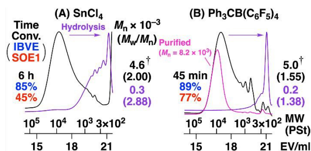
Figure 1. MWD curves of poly(IBVE-co-SOE1)s [entries (A) 2 and (B) 5 in Table 1; black: original product, pink: after purification by reprecipitation in methanol, purple: their acid hydrolysis products (hydrolysis after purification by reprecipitation). See the footnote of Table 1 for the polymerization conditions. [† The M_n values of the main portions (the MW region over approximately 10^3 ). The M_n values calculated from the whole region including oligomer regions are (A) 2.9 \times 10^3 and (B) 1.8 \times 10^3 .]
