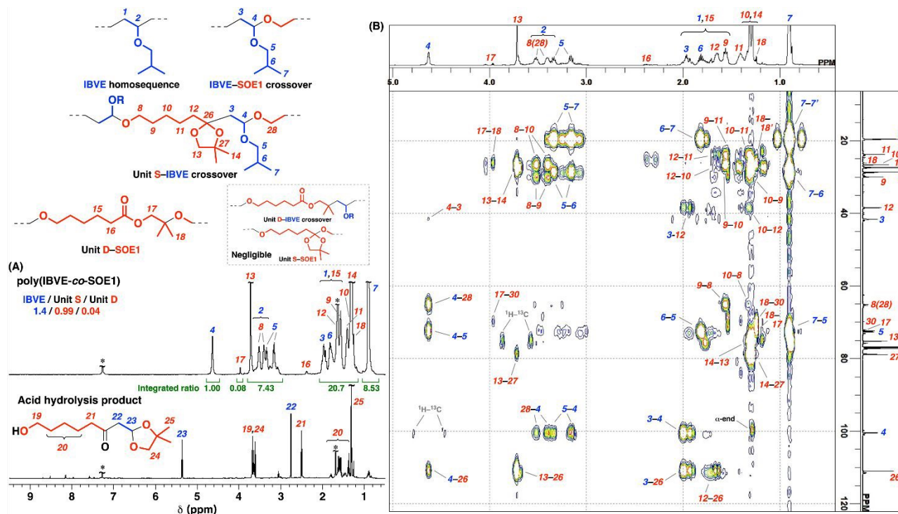
Figure 2. (A) ^1\text{H} NMR spectra of poly(IBVE-co-SOE1) (upper; entry 5 in Table 1; after purification by reprecipitation in methanol, a pink curve in Figure XB) and acid hydrolysis product (lower). (B) ^1\text{H} - ^{13}\text{C} HMBC NMR spectrum of poly(IBVE-co-SOE1) (entry 9 in Table 1; a limited region of the spectrum is shown; see Figure S9 for a wider region). See the footnote of Table 1 for the polymerization conditions. In \text{CDCl}_3 at 30 °C. * \text{CHCl}_3 or water.
