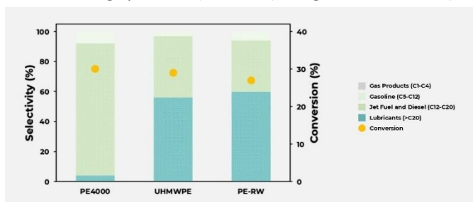
Figure 5: Comparison of mechanocatalytic upcycling of model PE4000, UHMWPE and real plastic waste promoted by Ru/Al 2 O 3 catalyst in the presence of 2-PrOH as H-donor source. Reaction conditions: room temperature, 6 h, PE/Ru mass ratio: 40:1, PE/2-PrOH molar ratio: 1:100, MM-500 mixer mill: 1 x 10 mm zirconia balls, 30 Hz. Reported selectivity refers exclusively to GC-detectable volatile products.
