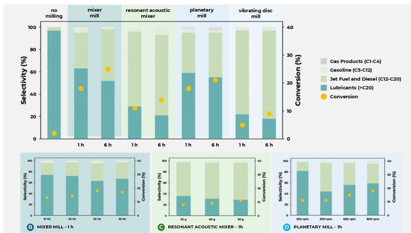
Figure 2: Influence of mechanical parameters on the PE4000 upcycling (conversion and product selectivity) without catalyst and without H-donor & LAG agent. (A) Comparative performance of the four mechanochemical systems as a function of reaction time (1–6 h). Reaction conditions: room temperature, 1–6 h, no catalyst, no H-donor, 1 \times 10 mm zirconia ball for Mixer Mill with 30 Hz frequency, no milling media for Resonant Acoustic Mixer with 90 g acceleration, 10 \times 10 mm zirconia ball for Planetary Mill with 800 rpm rotation speed, zirconia disc for Vibrating Disc Mill. (B) Effect of milling frequency in the MM-500 Mixer Mill. Reaction conditions: room temperature, 1 h, no catalyst, no H-donor, 1 \times 10 mm zirconia ball. (C) Effect of acceleration in the RAM II Resonant Acoustic Mixers. Reaction conditions: room temperature, 1 h, no catalyst, no H-donor, no milling media. (D) Effect of rotational speed in the P7 Planetary Mill. Reaction conditions: room temperature, 1 h, no catalyst, no H-donor, 10 \times 10 mm zirconia balls. Reported selectivity refers exclusively to GC-detectable volatile products.
