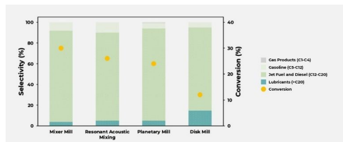
Figure 4: Comparative performance of four mechanochemical systems for the upcycling of PE4000 in the presence of Ru/Al 2 O 3 catalyst and 2-PrOH as H-donor source. Reaction conditions: room temperature, 6 h, PE/Ru mass ratio: 40:1, PE/2-PrOH molar ratio: 1:100, 1. MM-500 mixer mill: 1 x 10 mm zirconia balls, 30 Hz; P7 planetary mill: 10 x 10 mm zirconia balls, 800 rpm; RAM II resonant acoustic mixer: no milling media, 90 g acceleration; RS 300 disc mill: zirconia disc, default frequency. Reported selectivity refers exclusively to GC-detectable volatile products.
