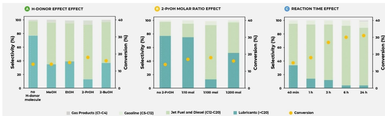
Figure 3: Effect of (A) the H-donor source, (B) the amount of 2-PrOH (PE/2-PrOH molar ratio), and (C) the reaction time, on the mechanocatalytic upcycling of PE4000 in the presence of Ru/Al 2 O 3 catalyst, in terms of both conversion and products selectivity. All reactions were performed using a mixer mill under the following conditions: room temperature, PE/Ru wt% ratio: 40:1, 1x10 mm zirconia ball, milling frequency = 30 Hz, reaction time = 1-6h, PE/2-PrOH molar ratio: 1:10-1:200. Reported selectivity refers exclusively to GC-detectable volatile products.
