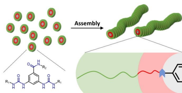
Figure 4: Schematic illustration of BDUA assembly induced by solvent exchange from THF to water through hydrophobic shielding.
