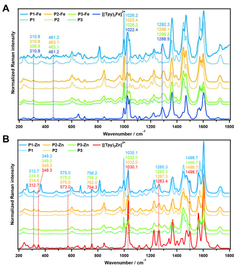
Fig. 5 Normalized FT-Raman spectra of the linear polymers P1 , P2 and P3 and (A) Fe-complexed and (B) Zn-complexed metallopolymers showing the band positions of the identified characteristic peaks for validation.
